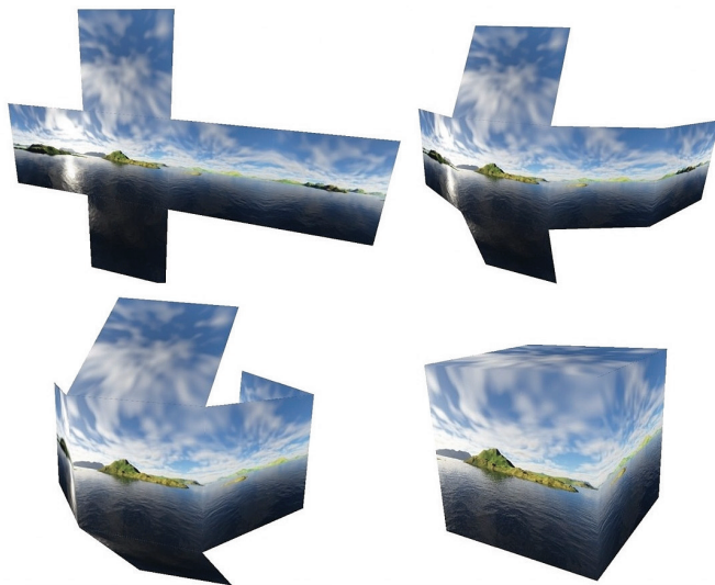
Figure 9.2 Texture cube map wrapping around the camera.
