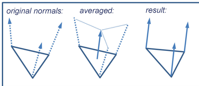
Figure 13.2 Applying averaged triangle surface normal to triangle vertices.
