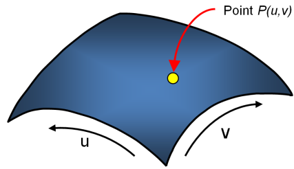
Figure 11.8 Parametric surface.
