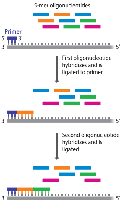
Figure 4.13 The basis to SOLiD sequencing. The mixture of 5-mer oligonucleotides (oligonucleotides that are five nucleotides in length) includes all 1024 possible sequences. The oligonucleotide that is complementary to the template DNA immediately adjacent to the primer hybridizes and is attached to the primer by DNA ligase. The cycle then repeats, resulting in hybridization and ligation of the second oligonucleotide.
