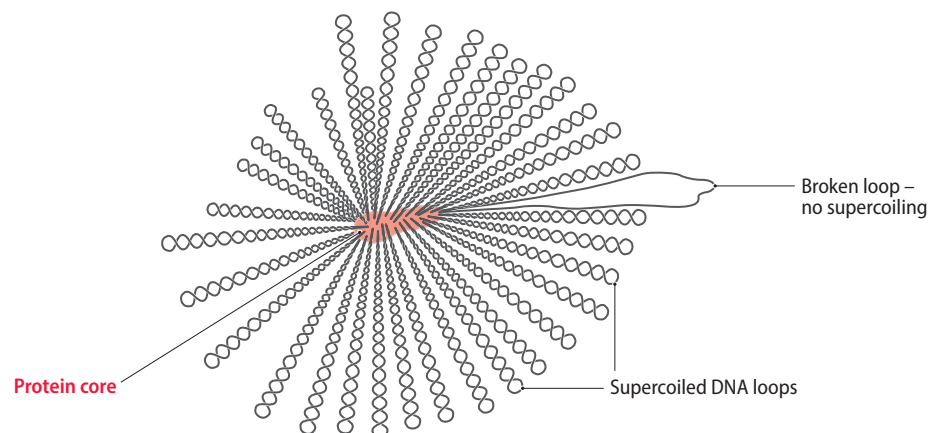
Figure 8.3 A model for the structure of the Escherichia coli nucleoid. Between 40 and 50 supercoiled loops of DNA radiate from the central protein core. One of the loops is shown in circular form, indicating that a break has occurred in this segment of DNA, resulting in a loss of supercoiling.
