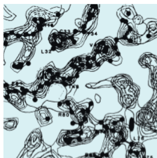
(A) Section of the ribonuclease electron density map
