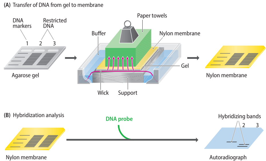
Figure 2.14 Southern hybridization.
