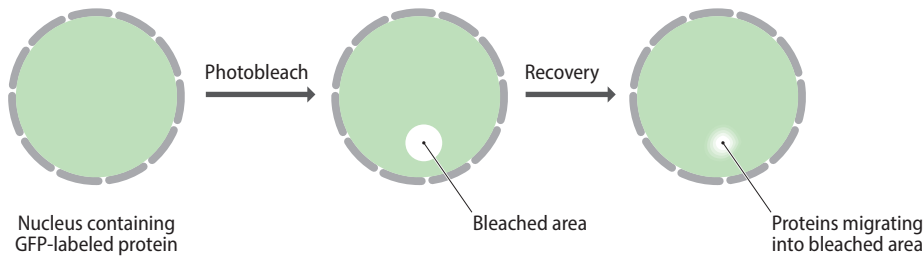
Figure 10.3 Fluorescence recovery after photobleaching (FRAP). A small area of a nucleus containing a fluorescently labeled protein is bleached by exposure to a laser beam. The migration of proteins into the bleached region from the unexposed area of the nucleus can then be observed.
