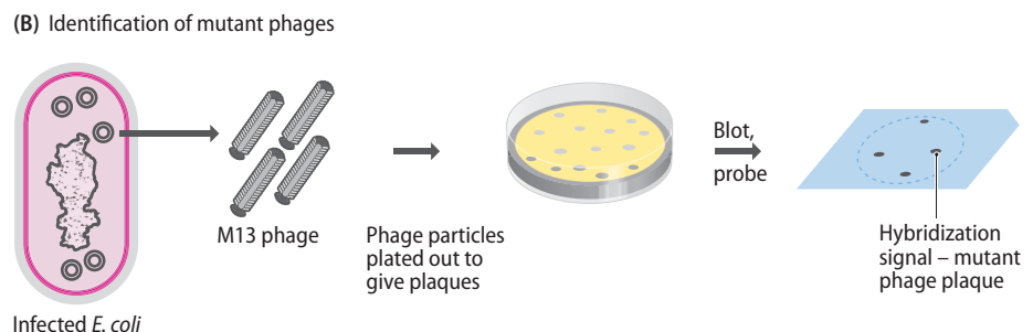
Figure 6.17 Oligonucleotide-directed mutagenesis. (A) A short oligonucleotide, containing a mismatch with the template DNA, is used to prime synthesis of the second DNA strand. (B) Replication in E. coli produces M13 phages containing a mixture of mutated and unmutated molecules. Plaques are blotted onto a membrane, and the ones containing the mutation are identified by hybridization probing with the original oligonucleotide.
