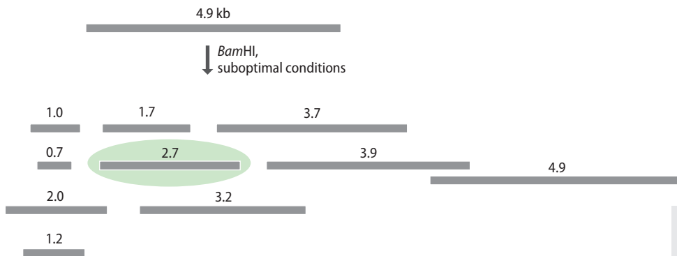
Figure 3.28 The conventional approach to restriction mapping. The objective is to map the Eco RI (E) and Bam HI (B) sites in a linear DNA molecule of size 4.9 kb. The results of single and double restrictions are shown at the top. The sizes of the fragments given after double restriction enable two alternative maps to be constructed, as explained in the central panel; the unresolved issue is the position of one of the three Bam HI sites. The two maps are tested by a partial Bam HI restriction (bottom), which shows that Map II is the correct one.
