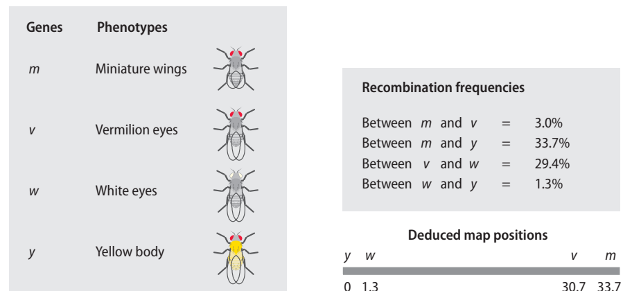
Figure 3.19 Working out a genetic map from recombination frequencies. The example is taken from the original experiments carried out with fruit flies by Arthur Sturtevant. All four genes are on chromosome 1 of the fruit fly. Recombination frequencies between the genes are shown, along with their deduced map positions.
