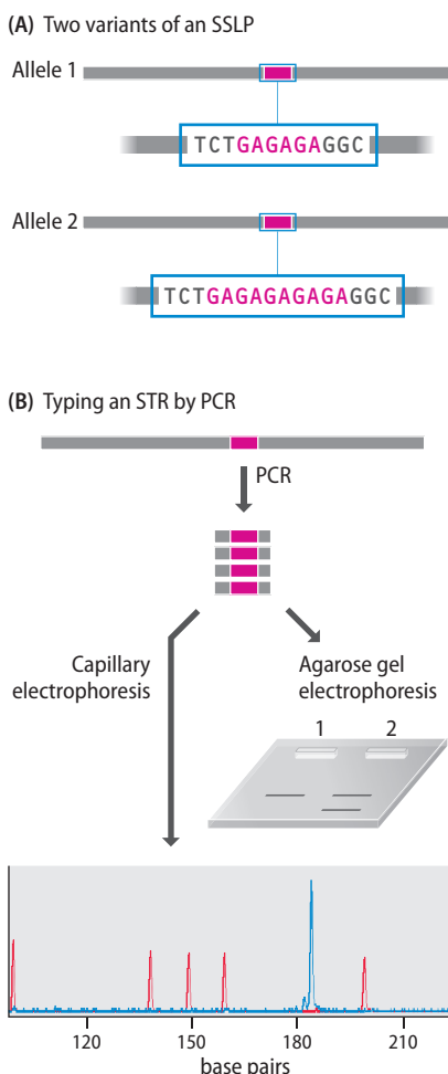
Figure 3.6 SSLPs and how they are typed. (A) Two alleles of an SSLP. This particular example is a short tandem repeat (STR), also called a microsatellite. In allele 1, the motif GA is repeated three times, and in allele 2, it is repeated five times. (B) Typing an STR by PCR. The STR and part of the surrounding sequence is amplified, and the size of the product is determined by agarose gel electrophoresis or capillary electrophoresis. In the agarose gel, lane 1 contains the PCR product and lane 2 contains DNA markers that show the sizes of the bands given after PCR of the two alleles. The band in lane 1 is the same size as the larger of the two DNA markers, showing that the DNA that was tested contained allele 2. The results of capillary electrophoresis are displayed as an electrophoretogram, where the position of the blue peak indicates the size of the PCR product. The electrophoretogram is automatically calibrated against size markers (red peaks) so the precise length of the PCR product can be calculated.
