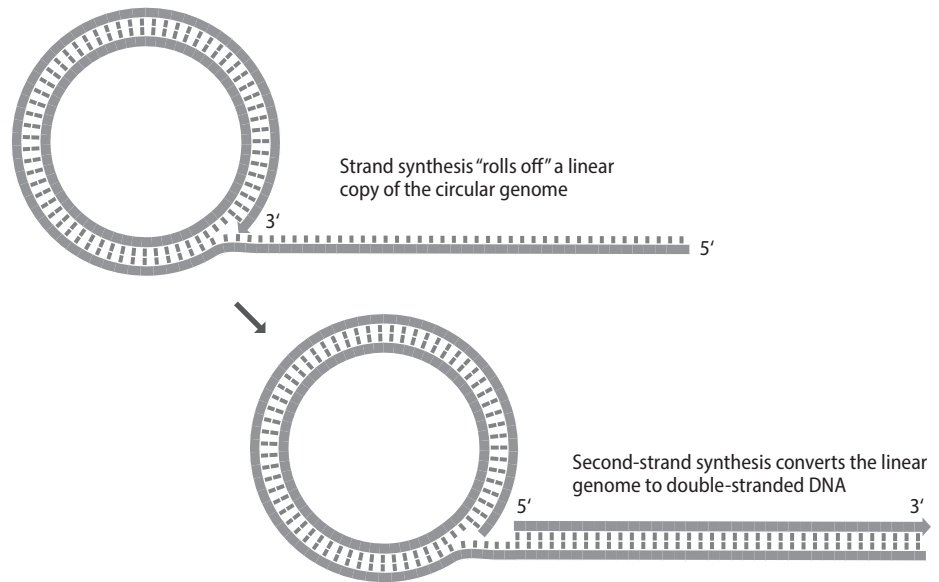
Figure 15.7 Rolling-circle replication.
