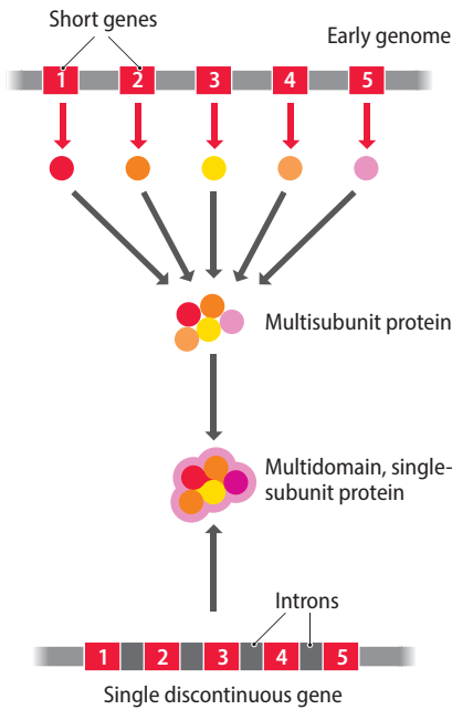
Figure 18.25 The exon theory of genes. The short genes of the first genomes probably coded for single-domain polypeptides that would have had to associate together to form a multisubunit protein and produce an effective enzyme. Later, the synthesis of this enzyme could have been made more efficient by linking the short genes together into one discontinuous gene coding for a multidomain single-subunit protein.
