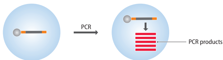
Figure 4.10 Amplification of immobilized libraries. (A) With the glass slide method, the fragment copies made by PCR attach to adjacent oligonucleotides, resulting in a cluster of identical immobilized fragments. (B) When metallic beads are used, PCR is carried out in the oil–water emulsion, and the fragment copies are retained in their individual water droplets.
