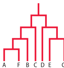
(B) Evolutionary relationships inferred from gene X sequences
