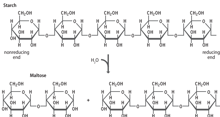
Figure 6.5 Mode of action of the enzyme specified by EC 3.2.1.2.
