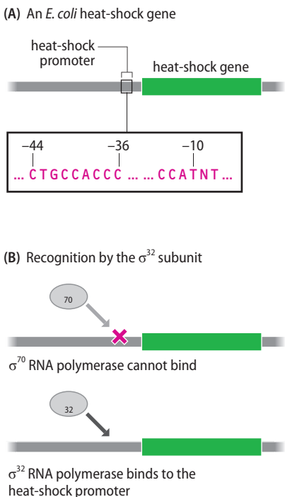
Figure 12.10 Regulation of gene expression by the \sigma^{32} subunit in E. coli . (A) Sequence of the promoter upstream of genes involved in the heat-shock response of E. coli . (B) The heat-shock promoter is not recognized by normal E. coli RNA polymerase containing the \sigma^{70} subunit, but it is recognized by the polymerase containing the \sigma^{32} subunit.
