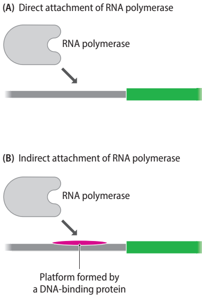
Figure 12.9 Two ways in which RNA polymerases bind to their promoters. (A) Direct recognition of the promoter by RNA polymerase, as occurs in bacteria. (B) Recognition of the promoter by a DNA-binding protein, which forms a platform onto which RNA polymerase binds.
