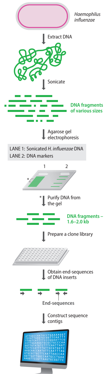
Figure 4.17 Shotgun sequencing of the Haemophilus influenzae genome.
