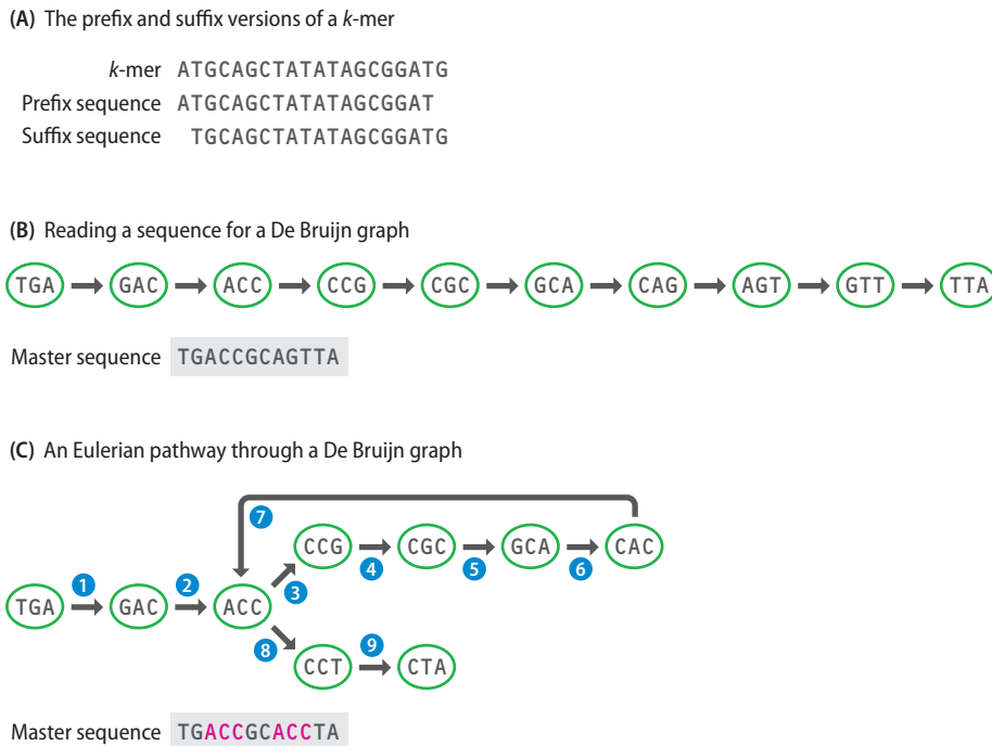
Figure 4.22 Sequence assembly by use of a De Bruijn graph. (A) A k -mer of 20 nucleotides and its prefix and suffix sequences. (B) An example of sequence assembly by use of a De Bruijn graph. In this example, the k -mers are just three nucleotides in length, which is too short for sequence assembly in the real world but serves to illustrate the principle of the method. Pairs of k -mers with identical suffix and prefix sequences have been identified: GA for the first two k -mers in the series and AC for k -mers 2 and 3. The edges, shown here as arrows, link pairs of k -mers, resulting in a series from which the master sequence can be read. (C) Sequences containing repetitive DNA regions can be assembled correctly from a De Bruijn graph if an Eulerian pathway through the graph can be identified. This is a pathway that visits every edge just once. In this example, the Eulerian pathway follows the edges labeled 1–9 in series, resulting in unambiguous assembly of the master sequence even though that sequence contains a repeat of the motif ACC
