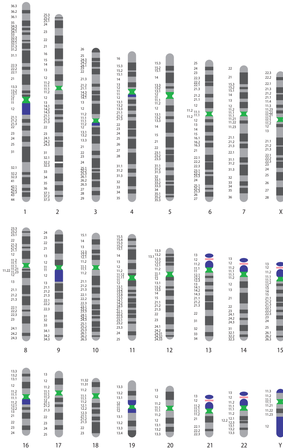
Figure 7.6 The human karyogram. The chromosomes are shown with their G-banding patterns. Chromosome numbers are given below each structure, and the band numbers are listed to the left. rDNA is a region containing a cluster of repeat units for the ribosomal RNA genes (Section 7.3). Constitutive heterochromatin is very compact chromatin that has few or no genes (Section 10.1).
