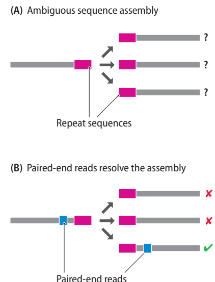
Figure 4.23 Using paired-end reads to resolve sequence assembly of a region that contains repetitive DNA. (A) In this example, the De Bruijn graph is ambiguous but identifies three segments of sequence that could be located downstream of a repeat sequence. (B) The locations of the paired-end reads obtained from a fragment that spans the repeat sequence identify which of the segments is positioned downstream of the repeat sequence.
