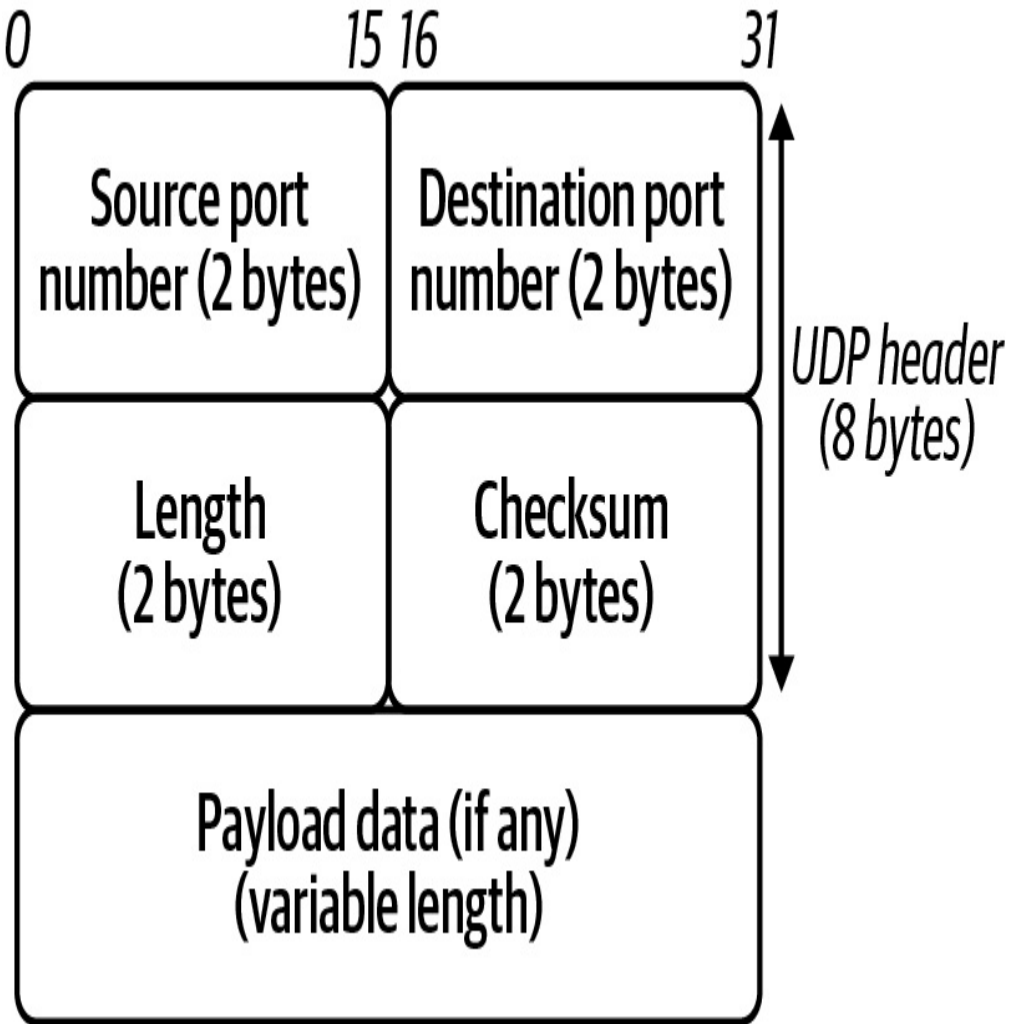
Figure 1-10. UDP header
