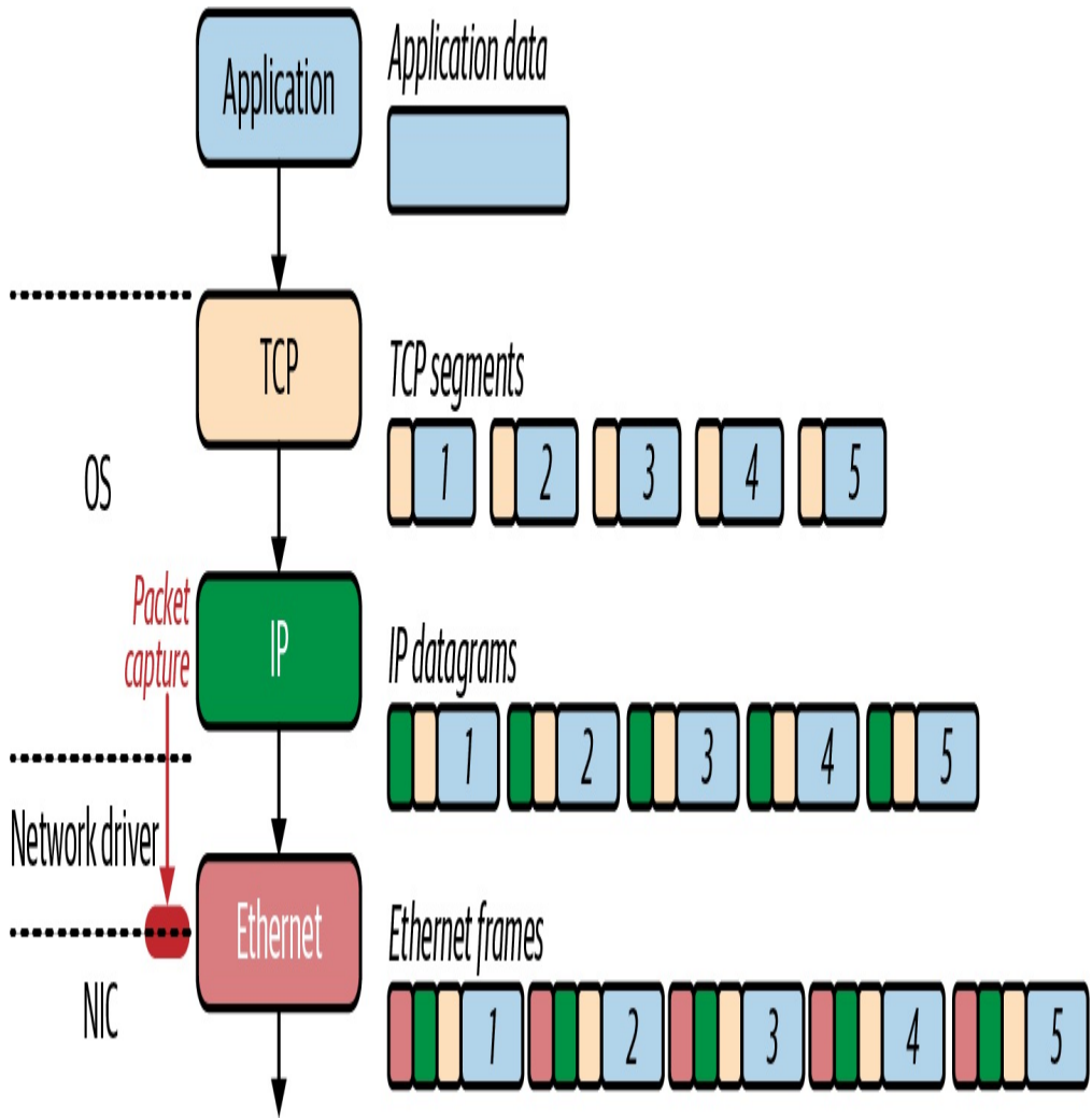
Figure 1-8. tcpdump packet capture
