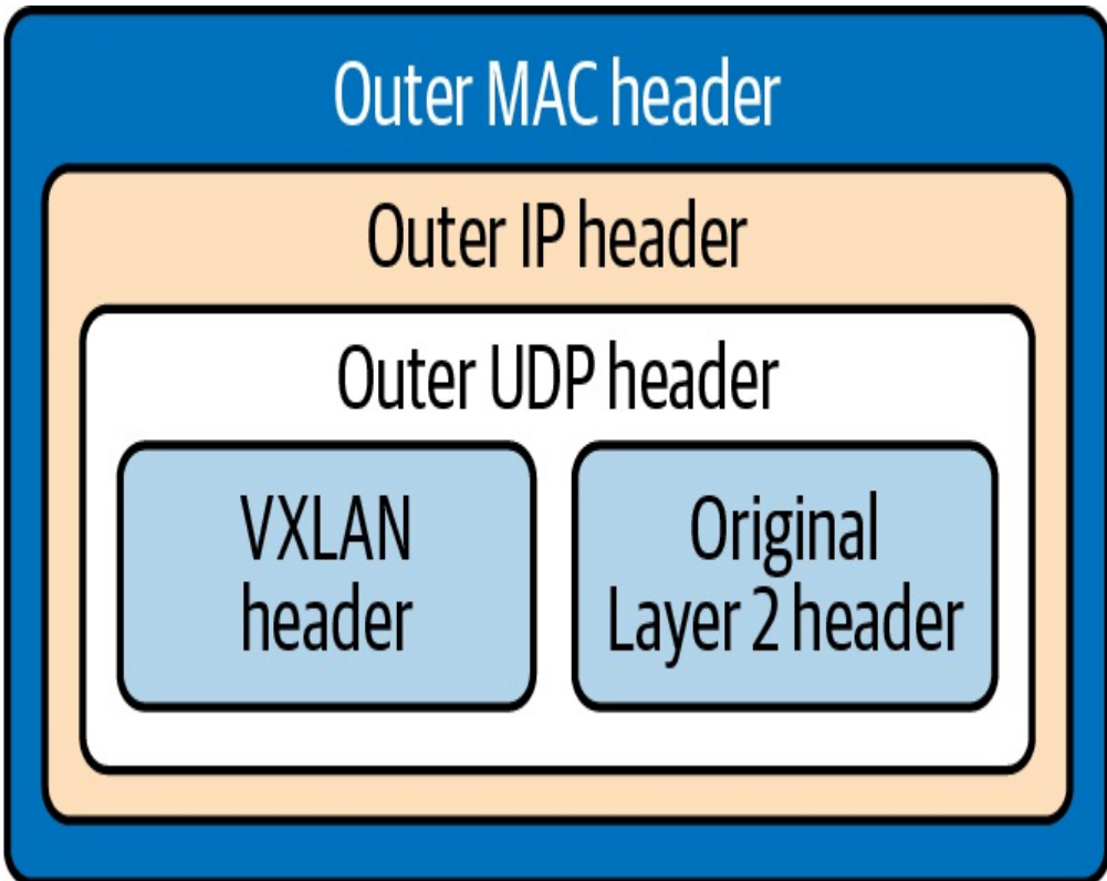
Figure 1-23. VXLAN packet
