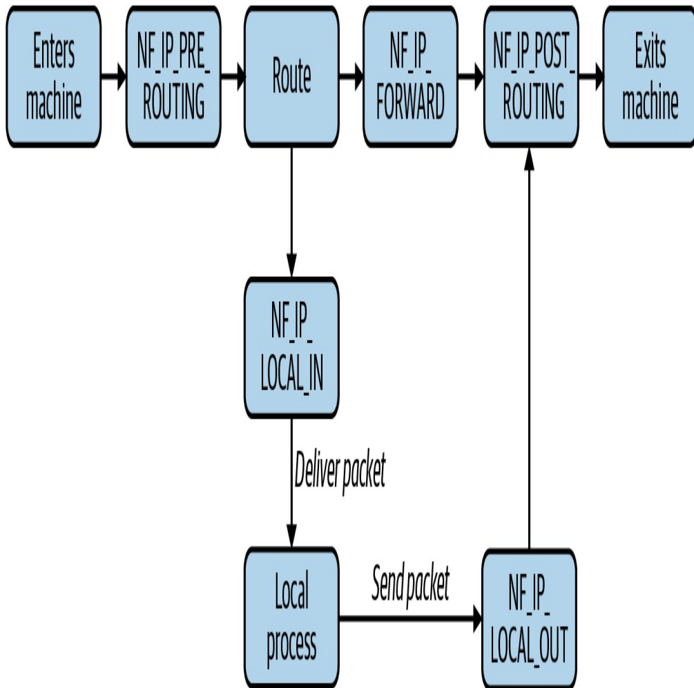
Figure 2-2. The possible flows of a packet through Netfilter hooks
