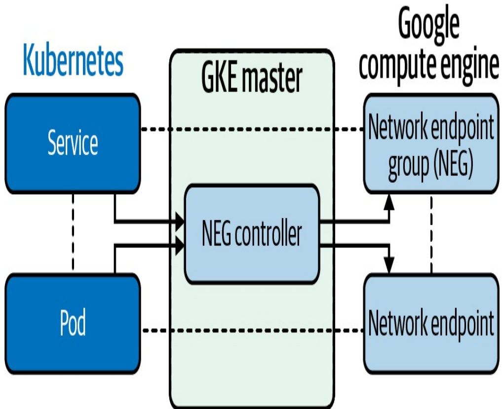
Figure 6-15. NEG to GCE components
