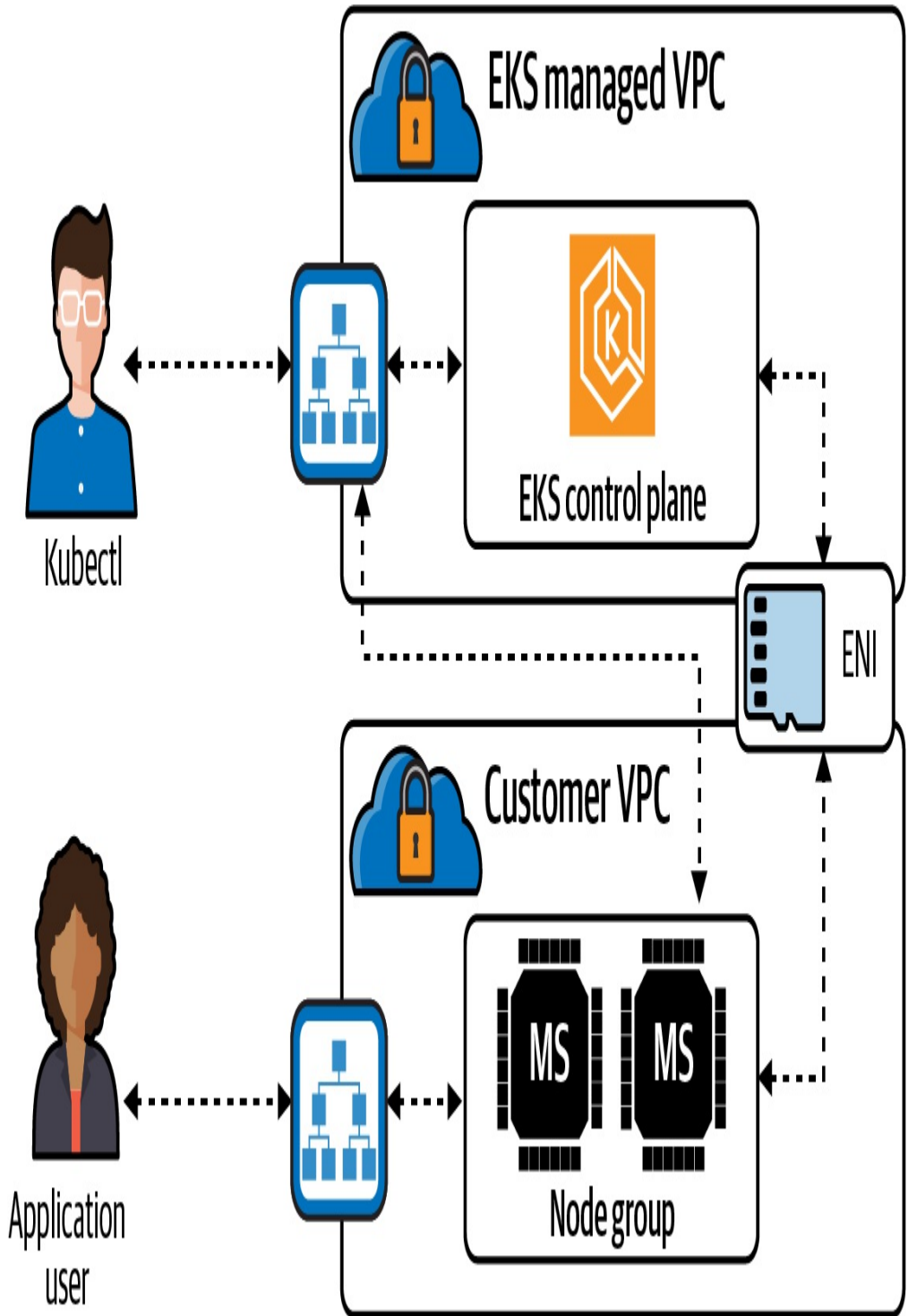
Figure 6-9. EKS communication path
