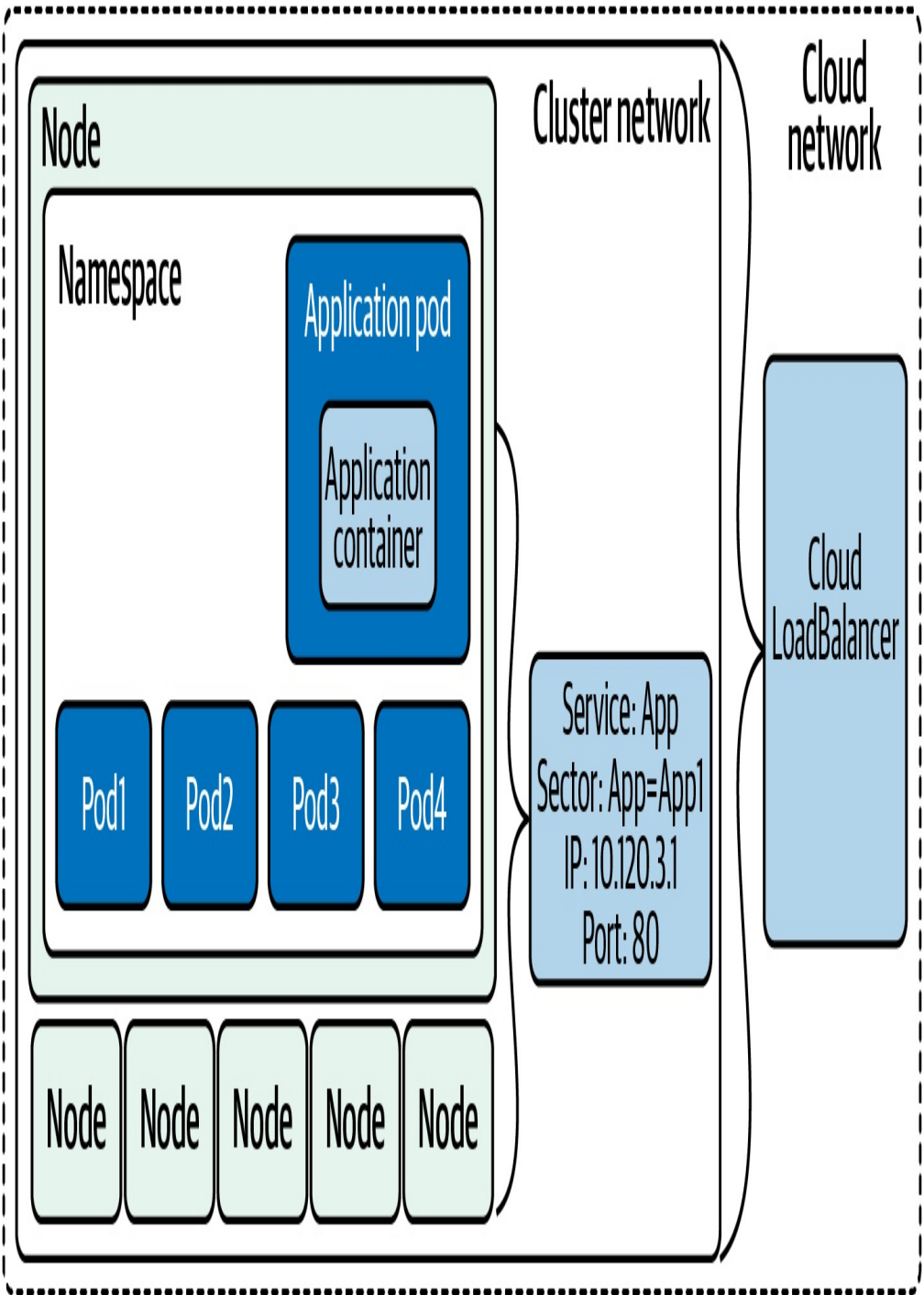
Figure 5-6. LoadBalancer service
