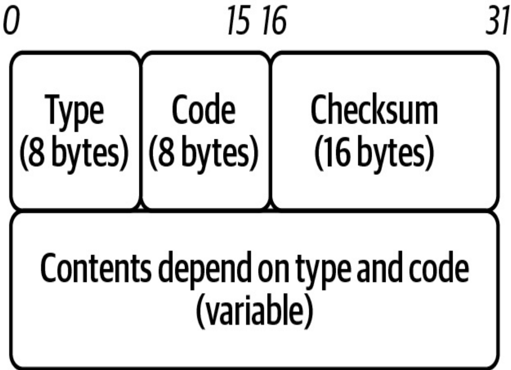
Figure 1-18. ICMP header
