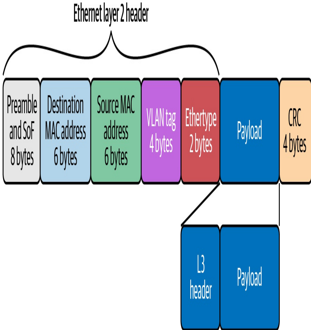
Figure 1-20. Ethernet header and footer
