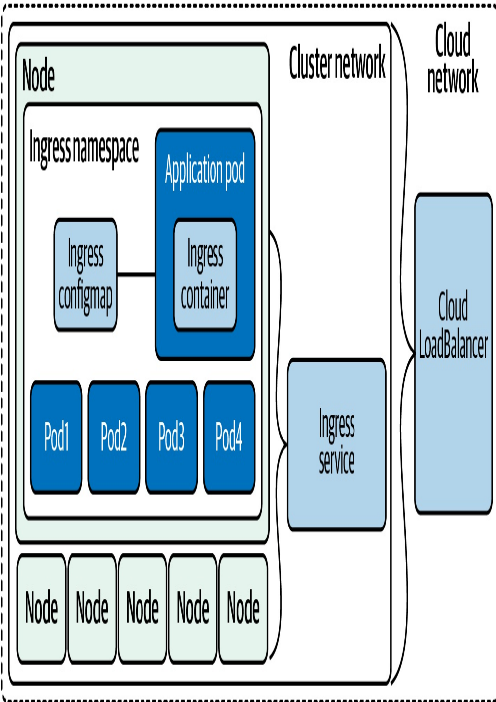
Figure 5-7. Ingress architecture
