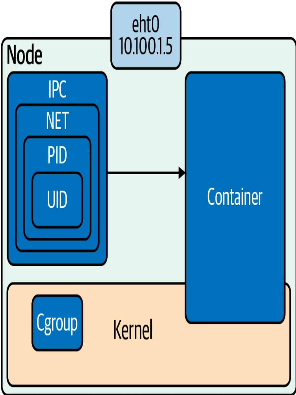
Figure 3-7. Cgroups and namespaces powers combined
