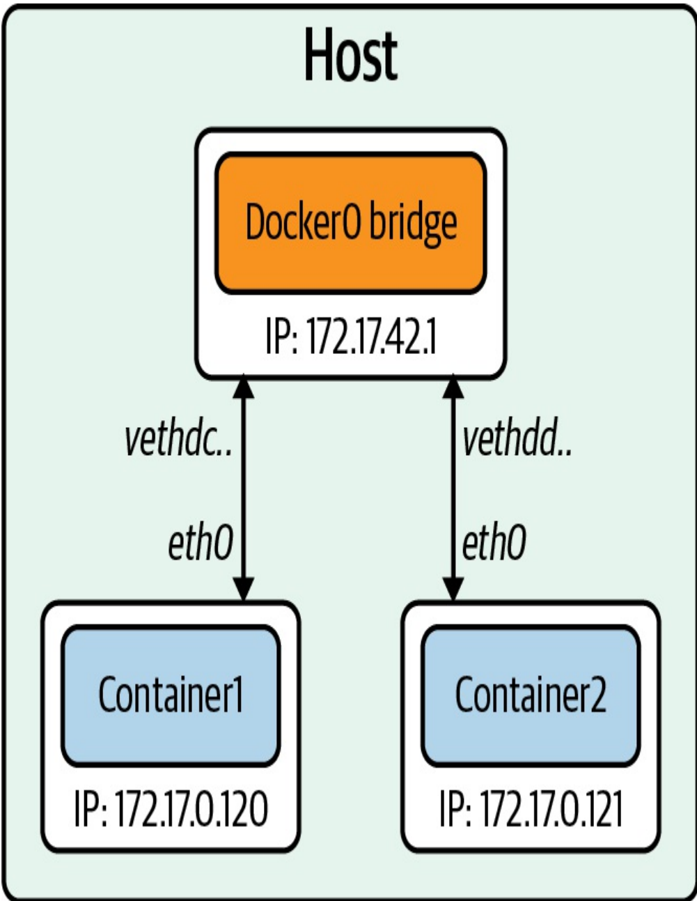
Figure 3-9. Docker bridge
