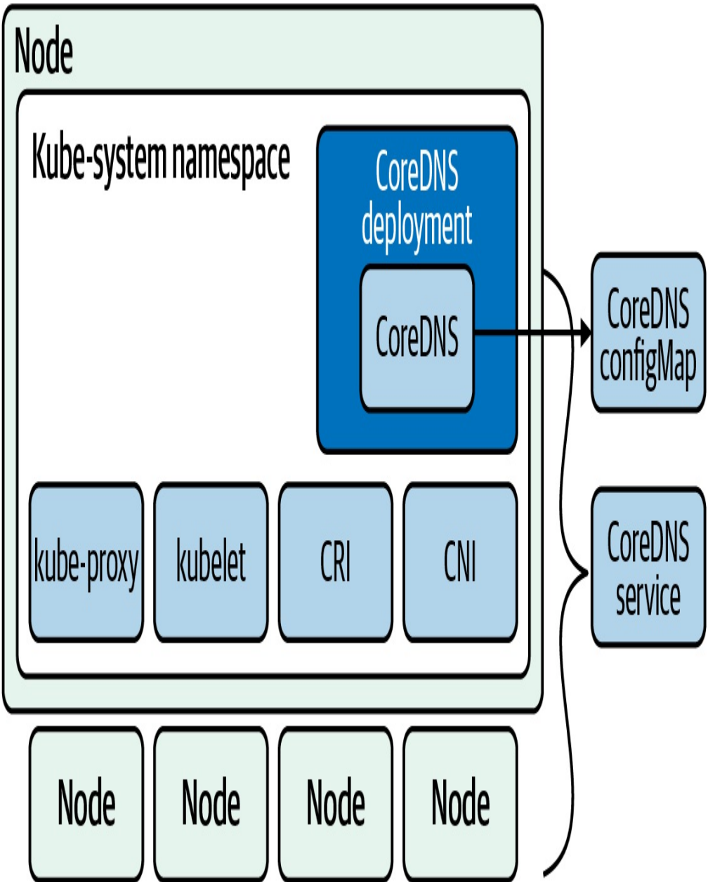
Figure 4-10. CoreDNS components
