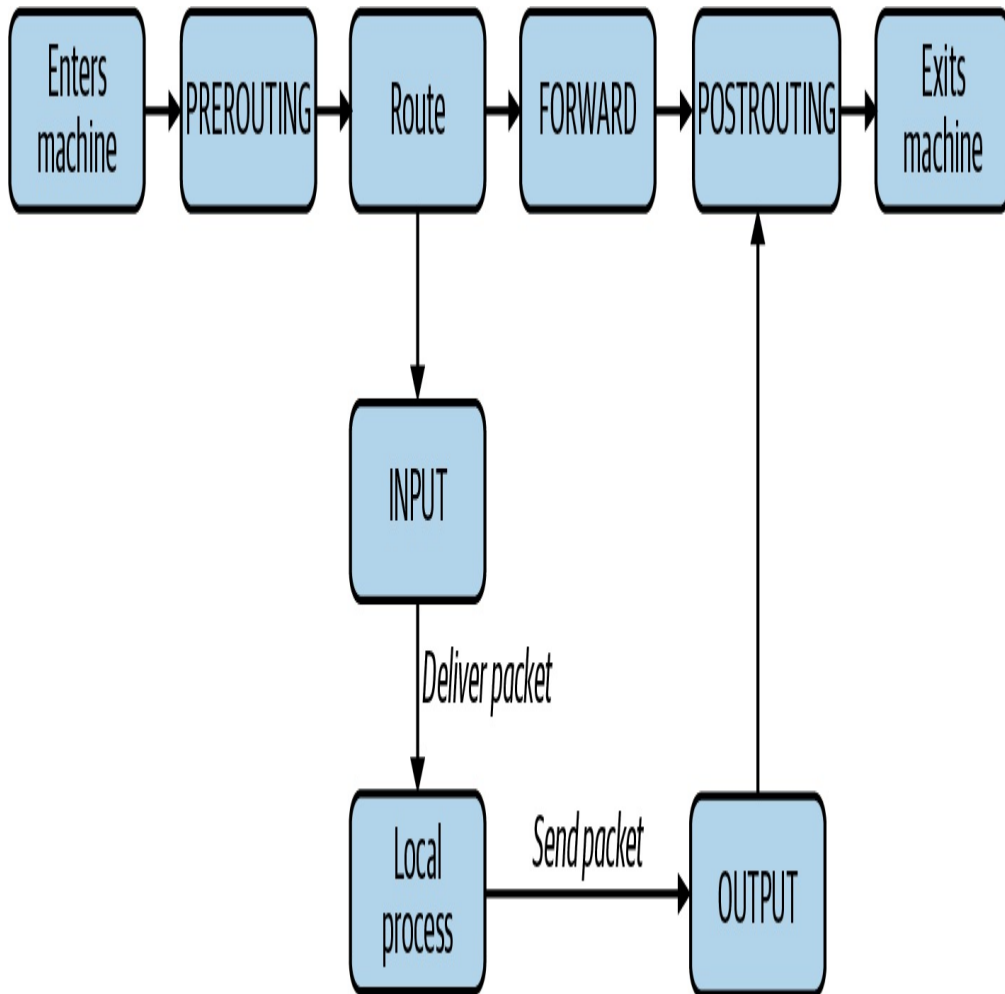
Figure 2-4. The possible flows of a packet through iptables chains
