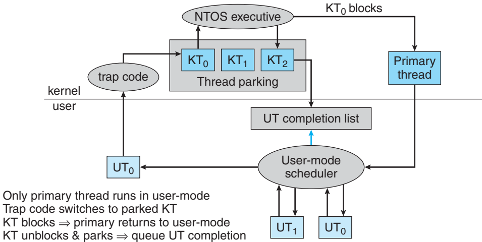
Figure 22.11 User-mode scheduling.
