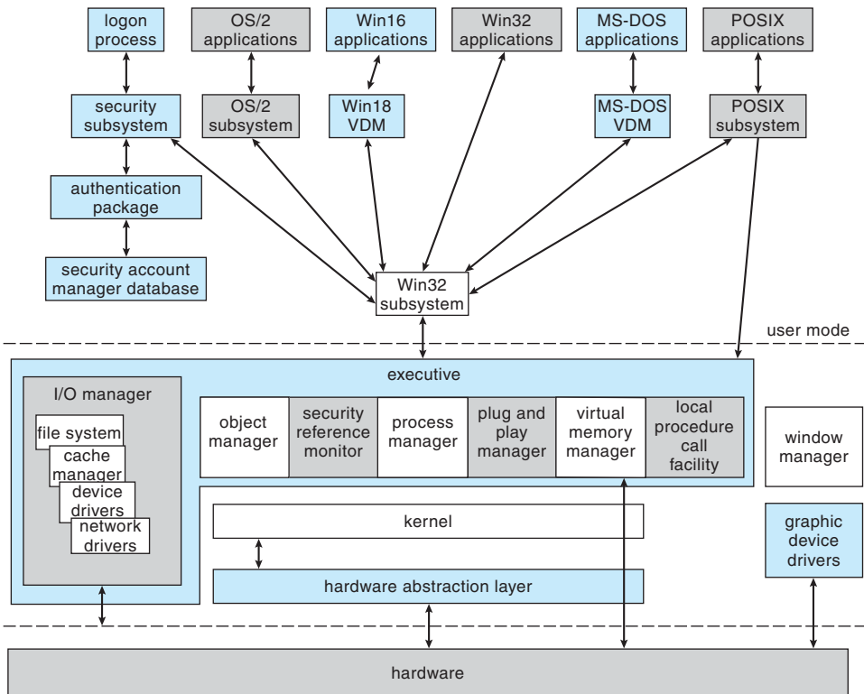
Figure 22.1 Windows block diagram.
