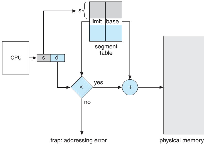
Figure 8.19 Segmentation hardware.
