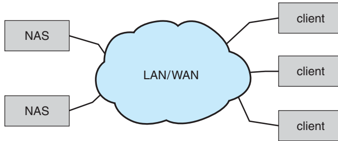
Figure 12.2 Network-attached storage.
