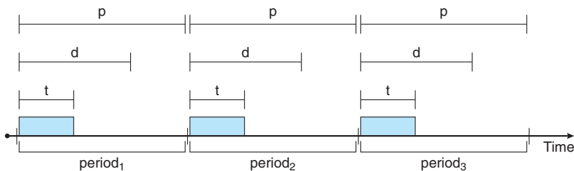
Figure 19.6 Periodic task.
