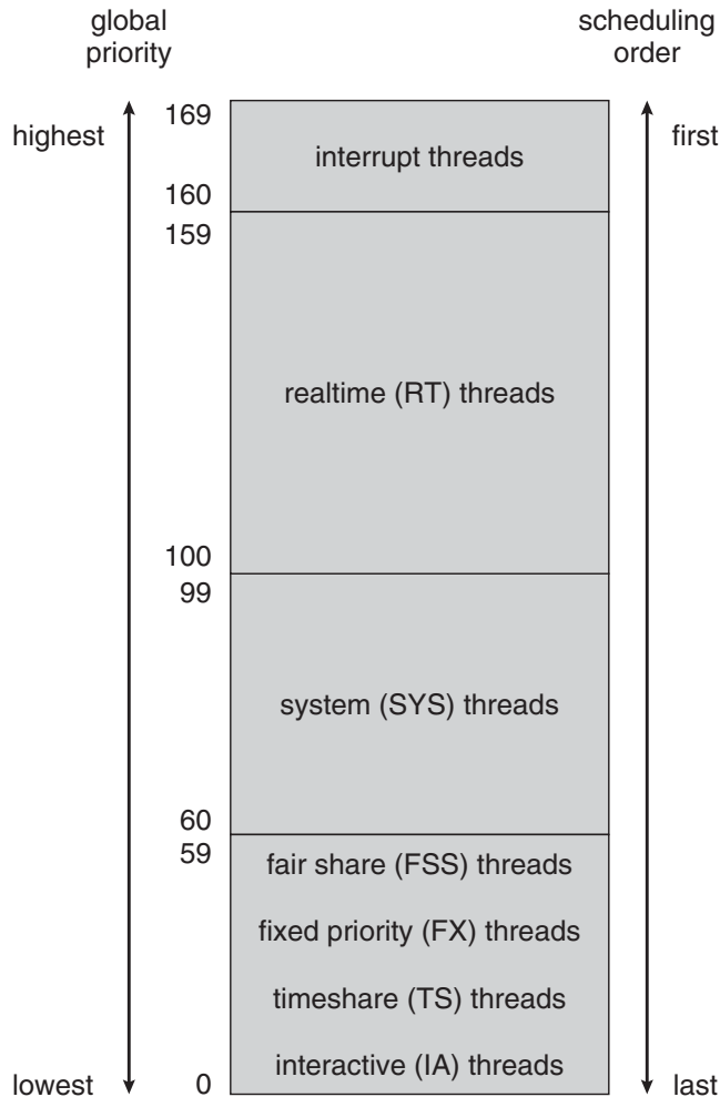
Figure 5.13 Solaris scheduling.
