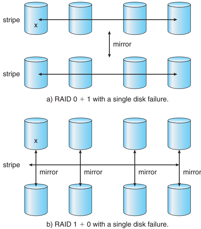
Figure 12.12 RAID 0 + 1 and 1 + 0.
