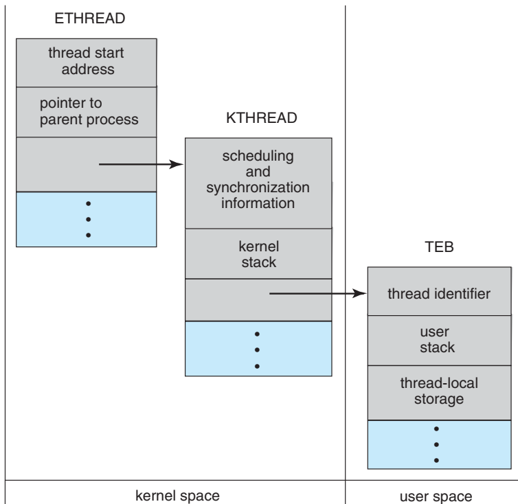
Figure 4.13 Data structures of a Windows XP thread.
