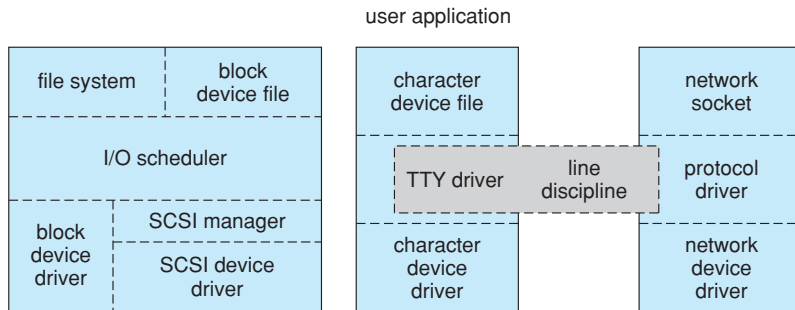
Figure 21.10 Device-driver block structure.
