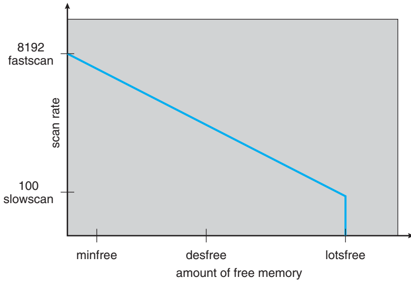
Figure 9.30 Solaris page scanner.
