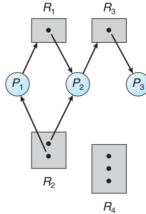
Figure 6.23 Resource-allocation graph.
