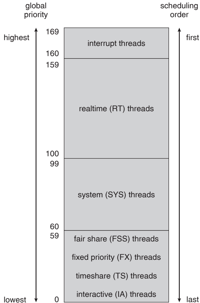
Figure 5.13 Solaris scheduling.
