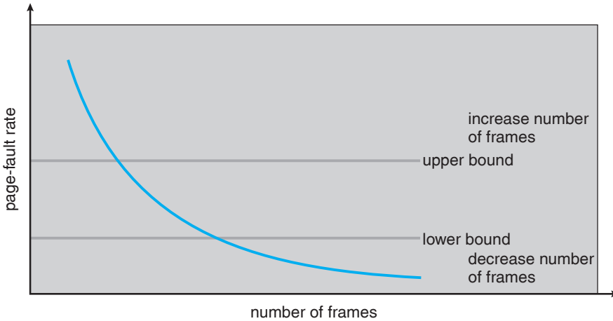
Figure 8.21 Page-fault frequency.
