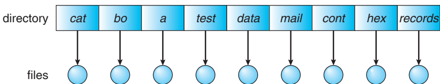
Figure 9.8 Single-level directory.
