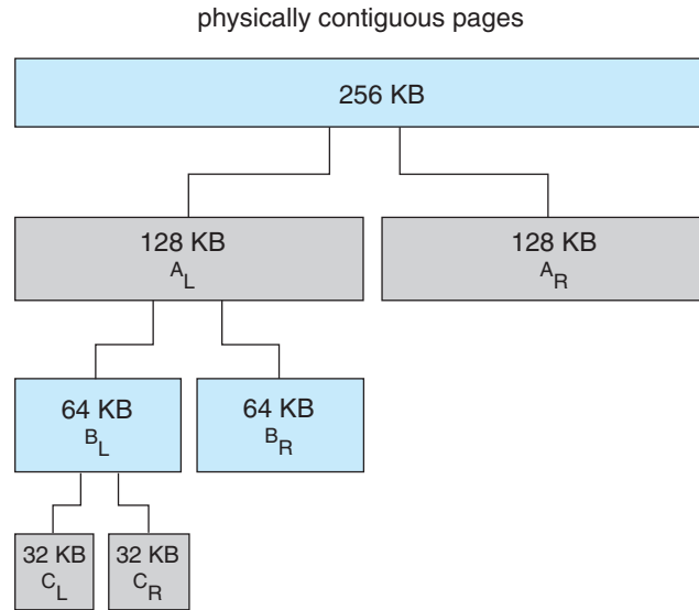
Figure 9.26 Buddy system allocation.
