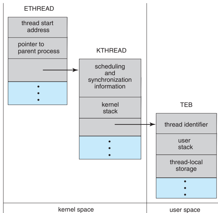
Figure 4.21 Data structures of a Windows XP thread.
