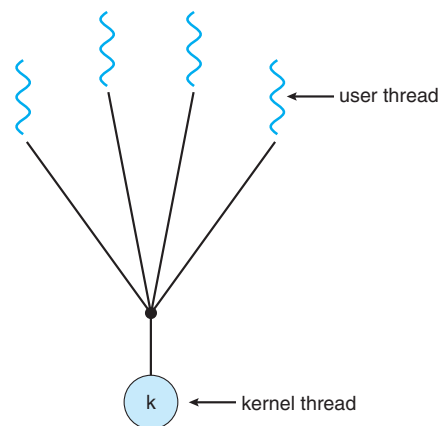
Figure 4.5 Many-to-one model.
