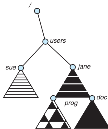
Figure 10.14 Mount point.
