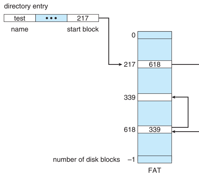
Figure 11.7 File-allocation table.
