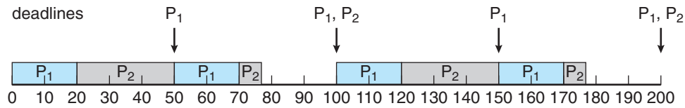
Figure 19.8 Rate-monotonic scheduling.
