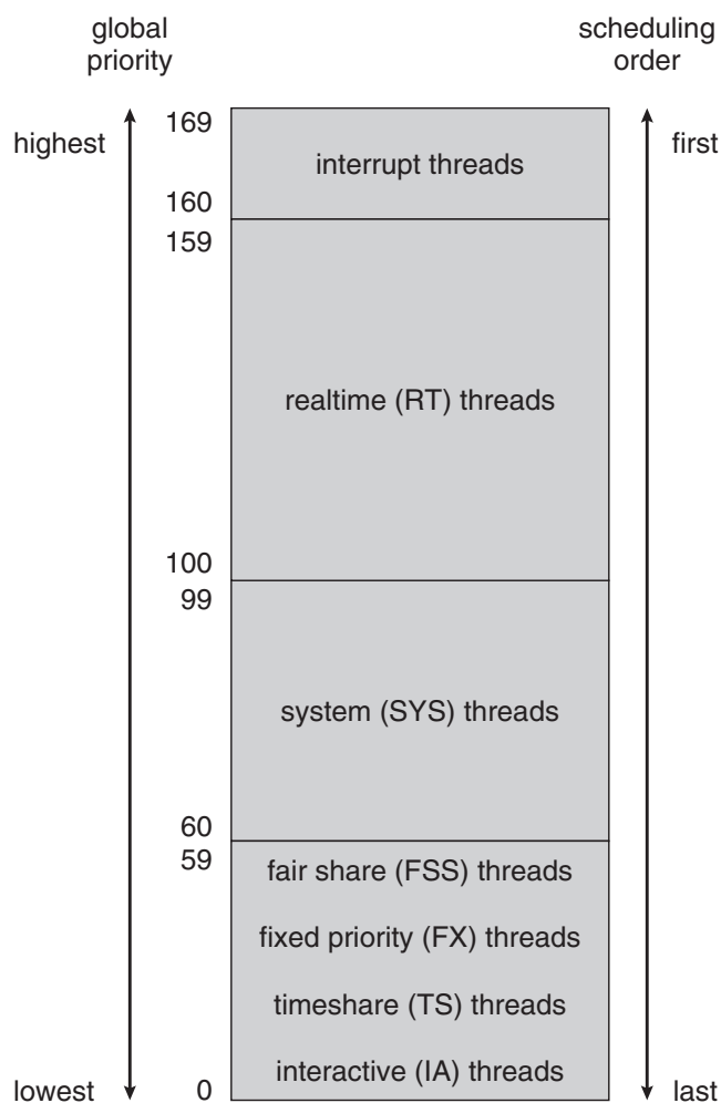
Figure 5.13 Solaris scheduling.
