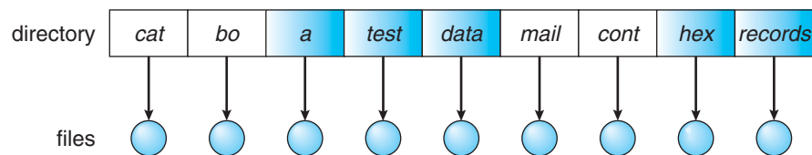
Figure 10.8 Single-level directory.
