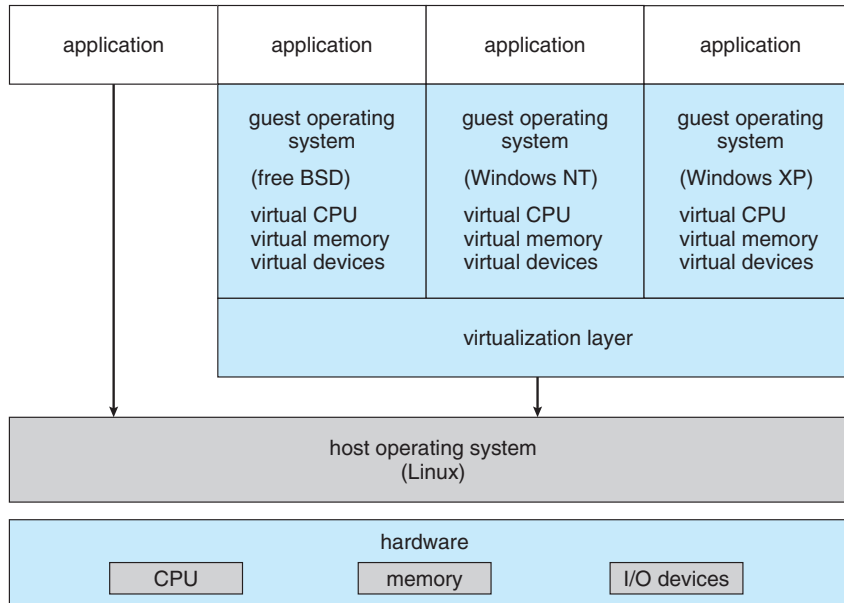
Figure 2.18 VMware architecture.
