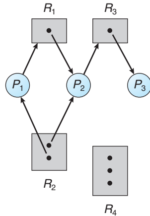
Figure 7.1 Resource-allocation graph.
