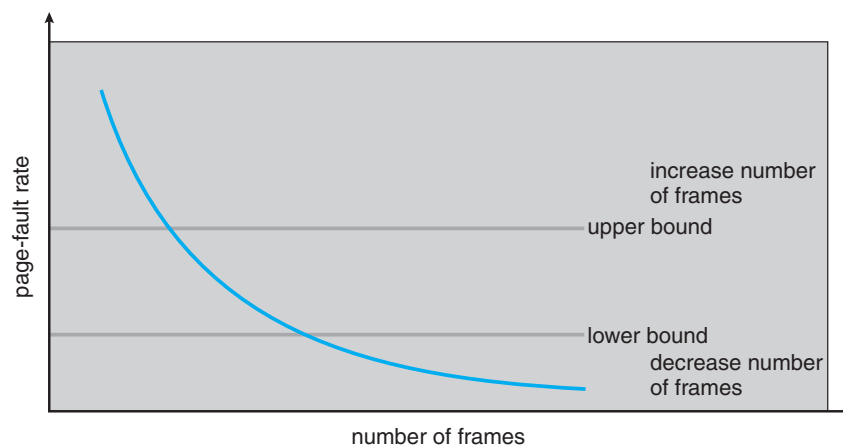
Figure 9.21 Page-fault frequency.
