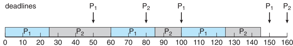
Figure 19.10 Earliest-deadline-first scheduling.
