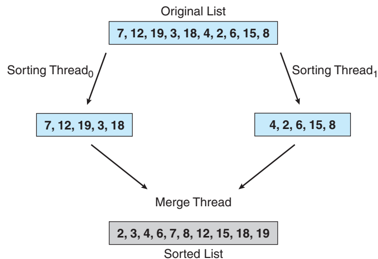
Figure 4.23 Sorting.
