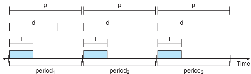
Figure 19.6 Periodic task.
