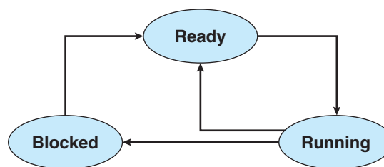
Figure 9.30 Thread state diagram for Exercise 9.15.
