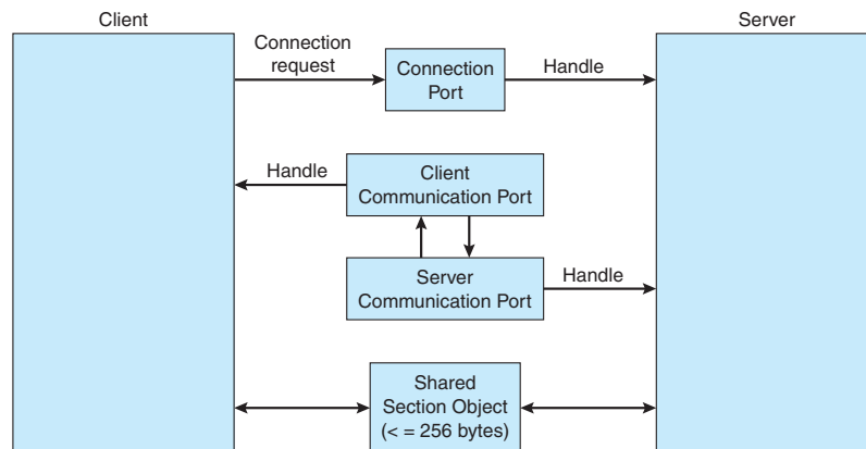
Figure 3.24 Local procedure calls in Windows XP.
