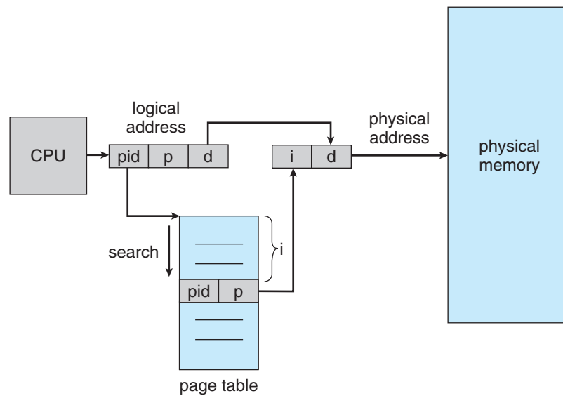
Figure 8.17 Inverted page table.
