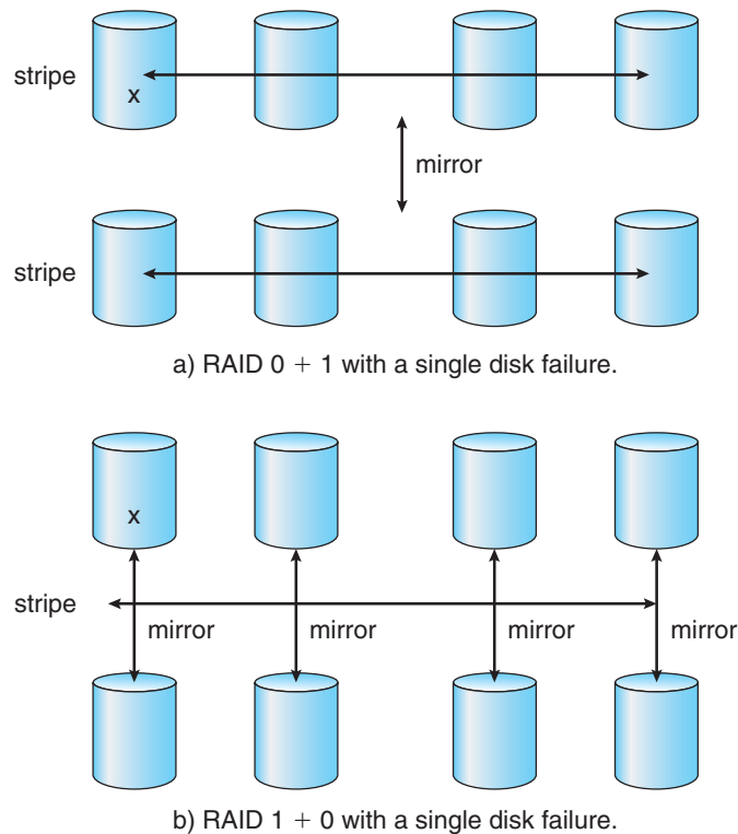
Figure 12.12 RAID 0 + 1 and 1 + 0.
