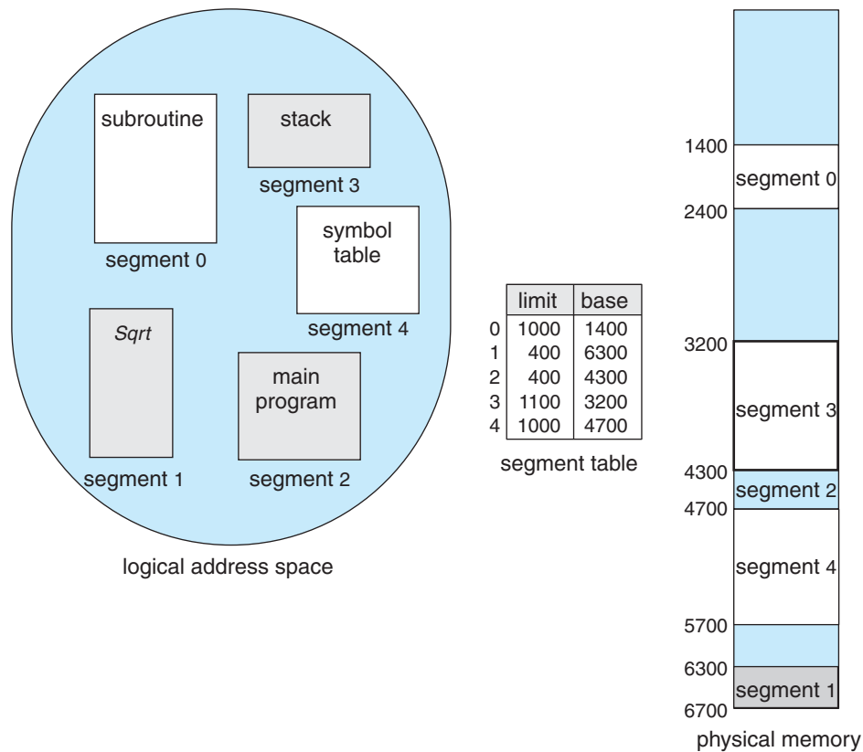
Figure 8.21 Example of segmentation.
