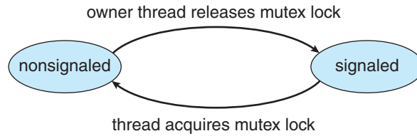
Figure 6.39 Mutex dispatcher object.
