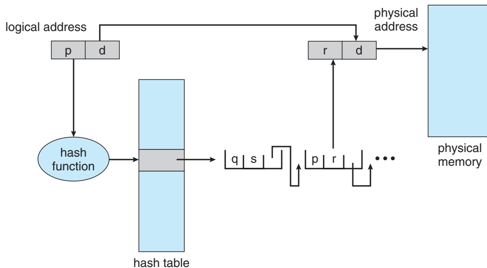
Figure 8.16 Hashed page table.
