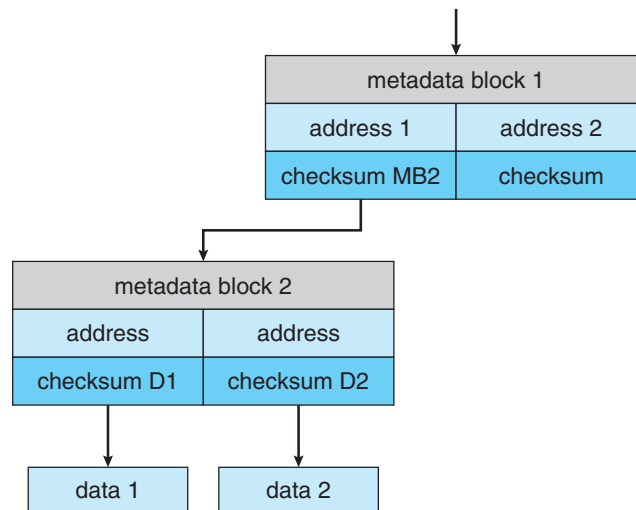
Figure 12.13 ZFS checksums all metadata and data.
