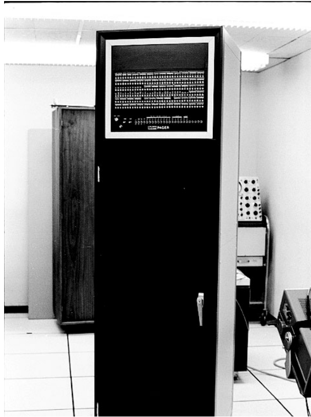
Figure 23.6 The BBN hardware-pager addition to the PDP-10.
