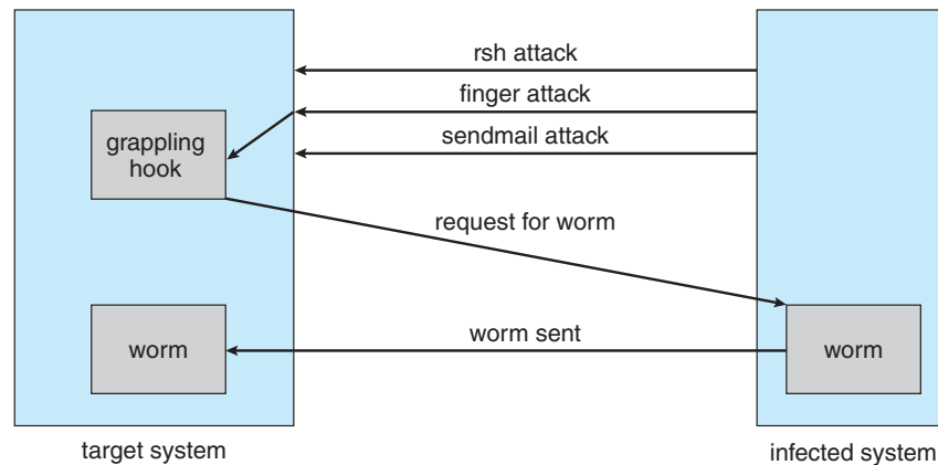
Figure 15.6 The Morris Internet worm.
