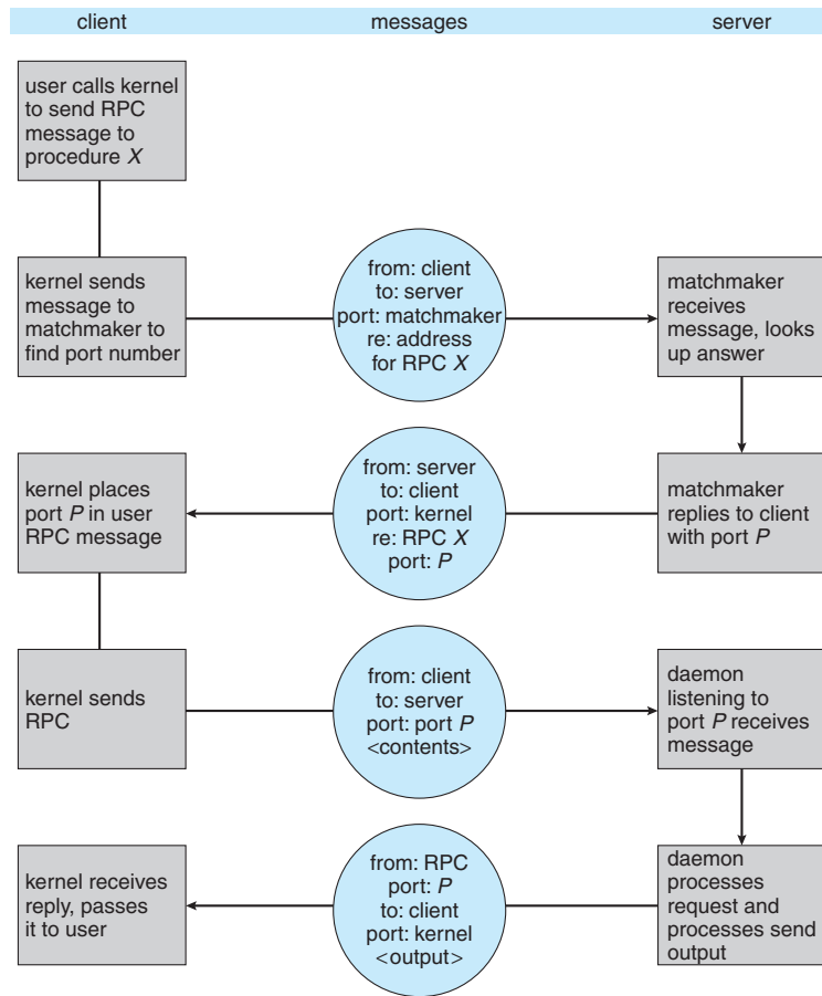
Figure 3.28 Execution of a remote procedure call (RPC).
