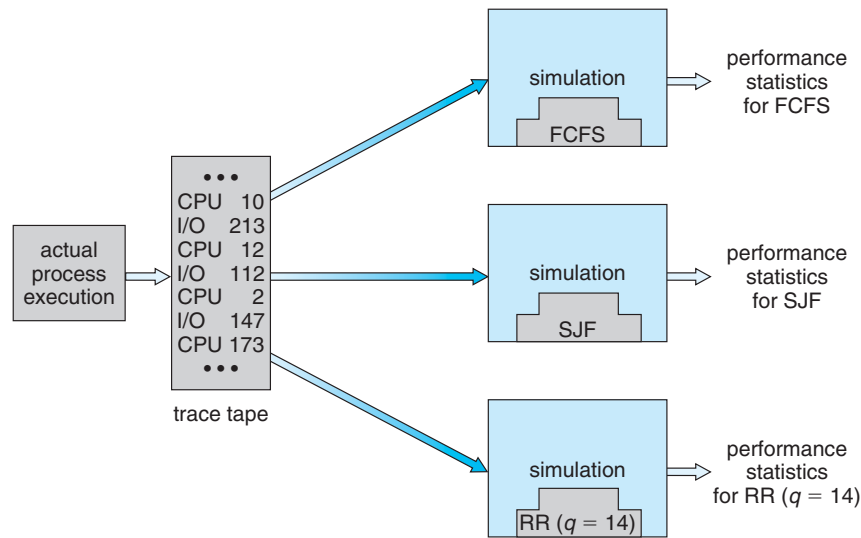
Figure 5.21 Evaluation of CPU schedulers by simulation.
