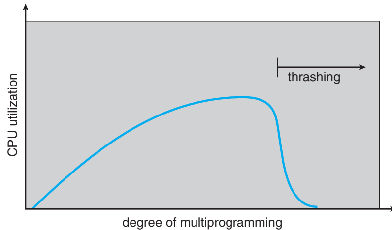
Figure 9.18 Thrashing.
