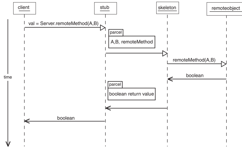
Figure 3.30 Marshalling parameters.
