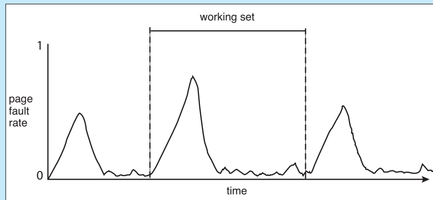
Figure 9.22 Page-fault rate over time.
