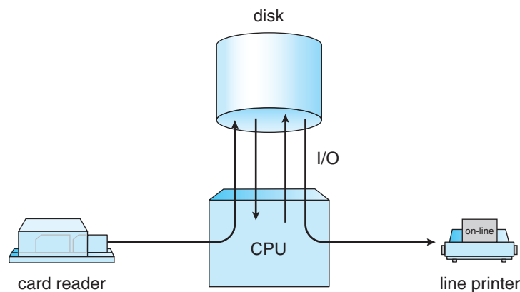
Figure 23.5 Spooling.
