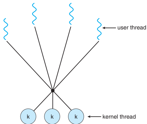
Figure 4.7 Many-to-many model.
