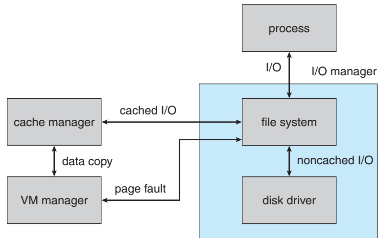
Figure 22.6 File I/O.
