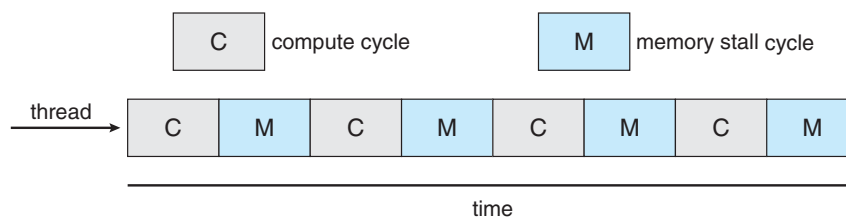
Figure 5.10 Memory stall.
