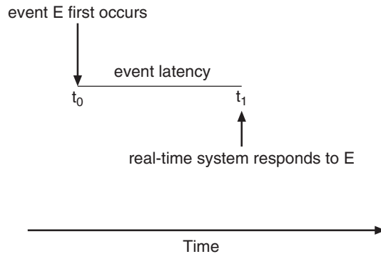
Figure 19.3 Event latency.
