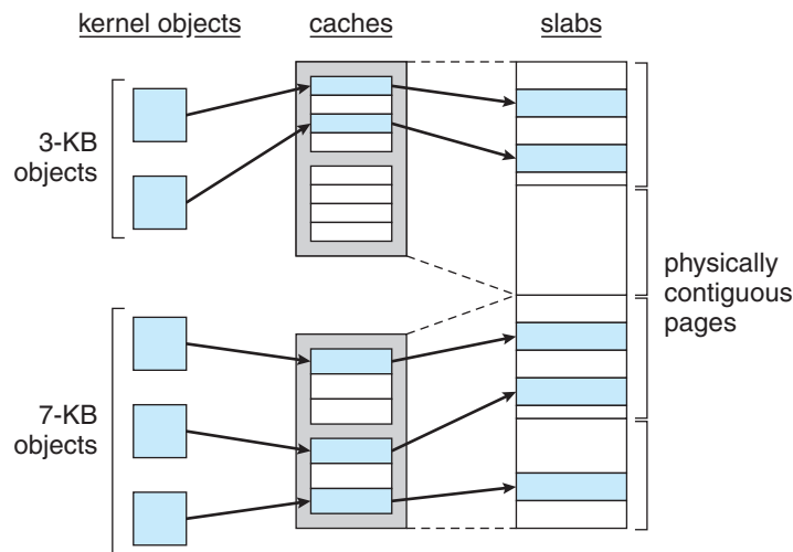
Figure 9.27 Slab allocation.
