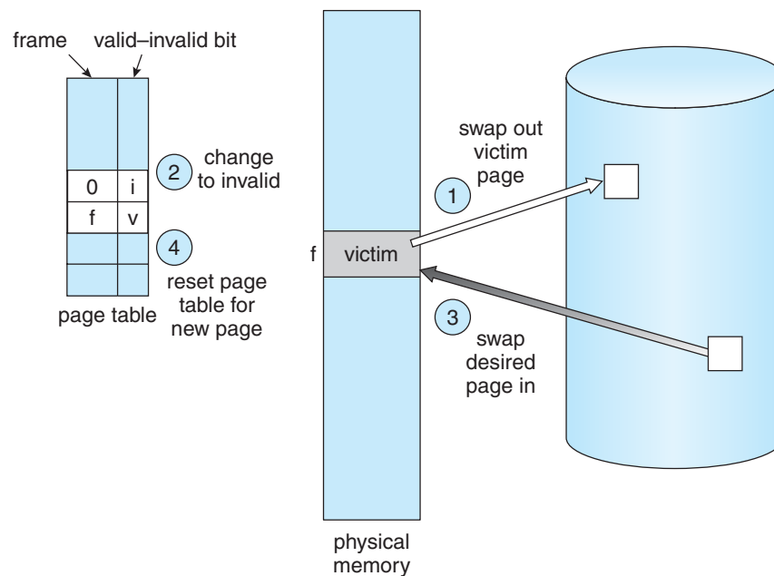
Figure 9.10 Page replacement.
