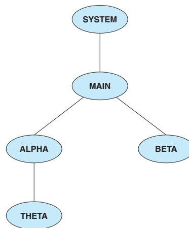
Figure 4.24 Thread-group hierarchy.
