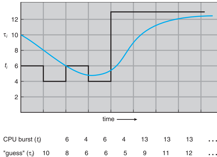
Figure 5.3 Predicting the length of the next CPU burst.
