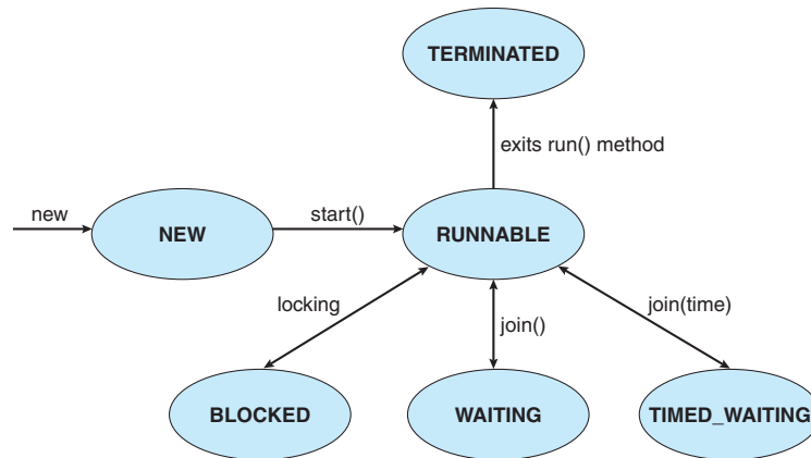
Figure 4.12 Java thread states.
