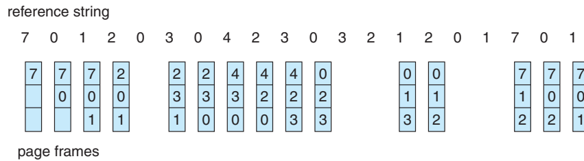
Figure 9.12 FIFO page-replacement algorithm.
