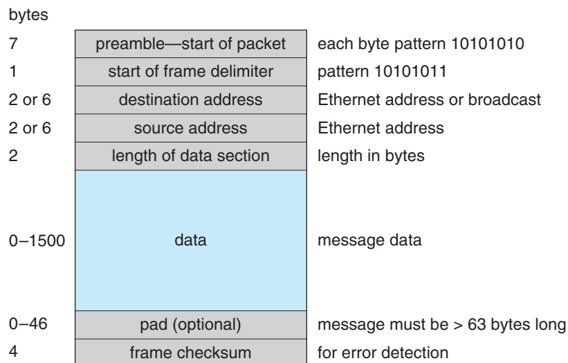
Figure 16.10 An Ethernet packet.
