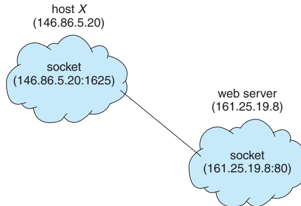
Figure 3.25 Communication using sockets.
