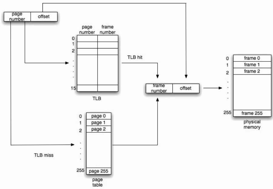
Figure 9.34 A representation of the address translation process.
