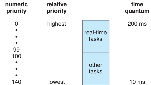
Figure 5.15 The relationship between priorities and time-slice length.
