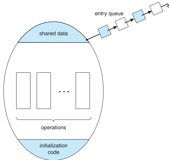
Figure 6.24 Schematic view of a monitor.
