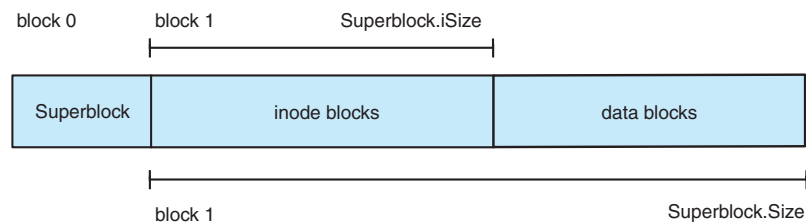
Figure 11.18 Structure of the simulated disk.
