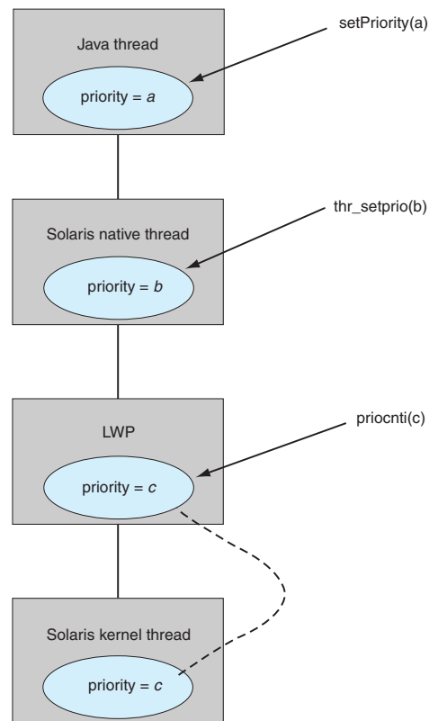
Figure 5.19 User threads are mapped to kernel threads through a lightweight process.
