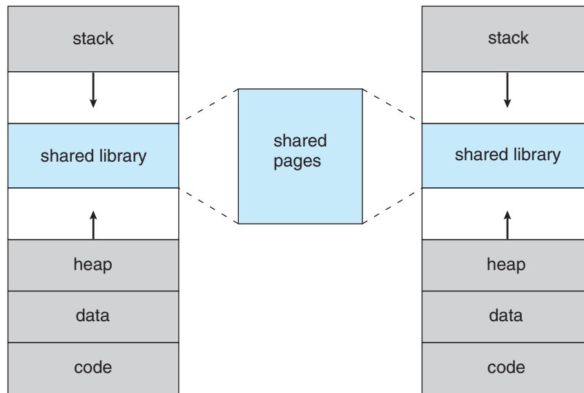
Figure 9.3 Shared library using virtual memory.
