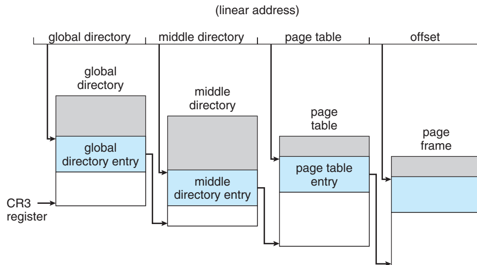
Figure 8.24 Three-level paging in Linux.
