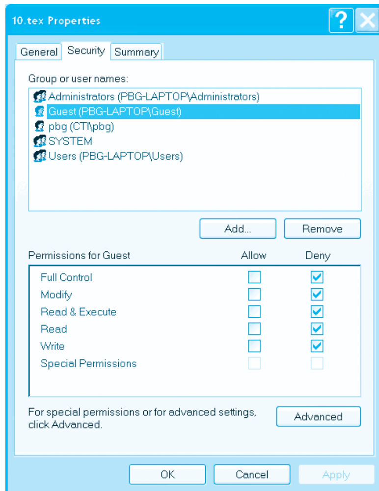
Figure 10.15 Windows XP access-control list management.
