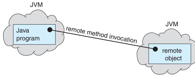
Figure 3.29 Remote method invocation.
