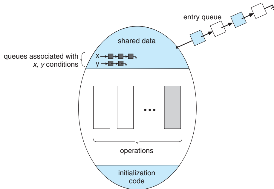
Figure 6.25 Monitor with condition variables.
