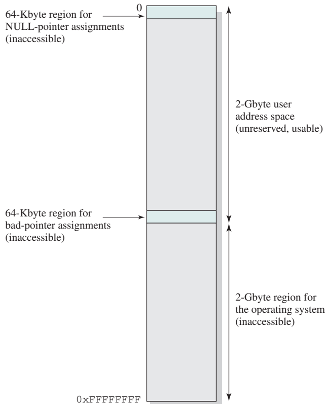
Figure 8.25 Windows Default 32-Bit Virtual Address Space
