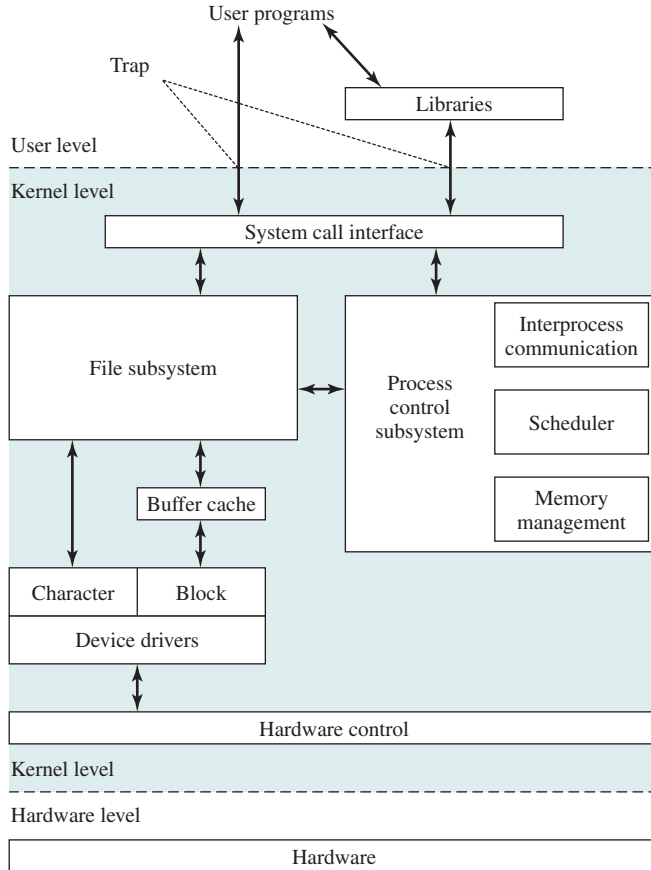
Figure 2.16 Traditional UNIX Kernel
