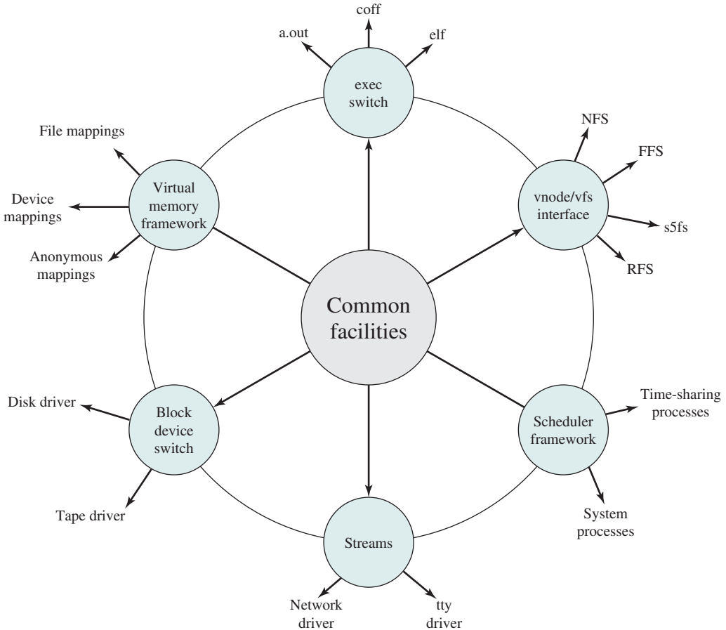
Figure 2.17 Modern UNIX Kernel
