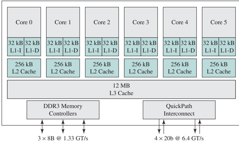
Figure 1.20 Intel Core i7-990X Block Diagram
