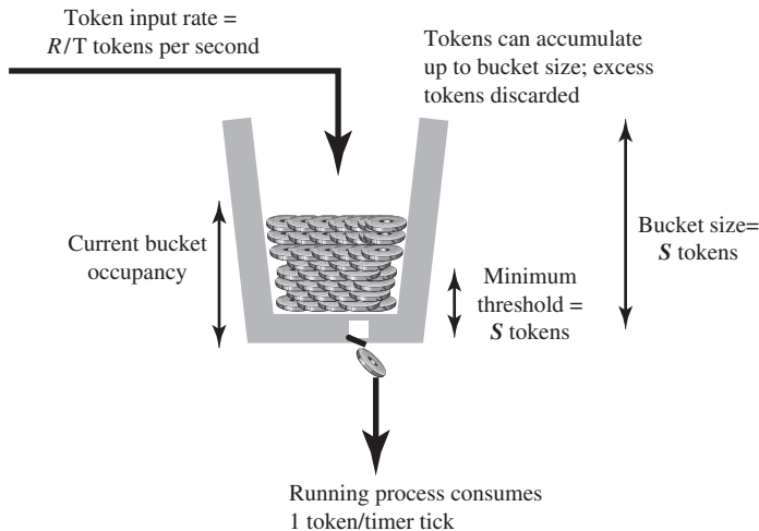
Figure 14.11 Linux VServer Token Bucket Scheme
