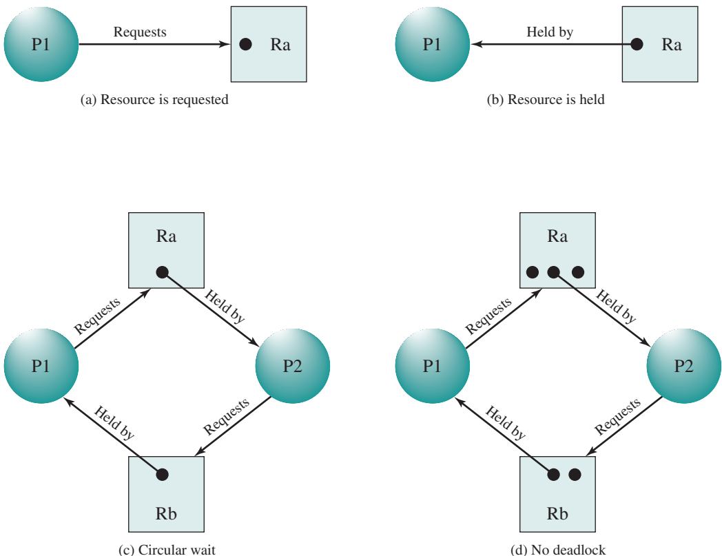
Figure 6.5 Examples of Resource Allocation Graphs
