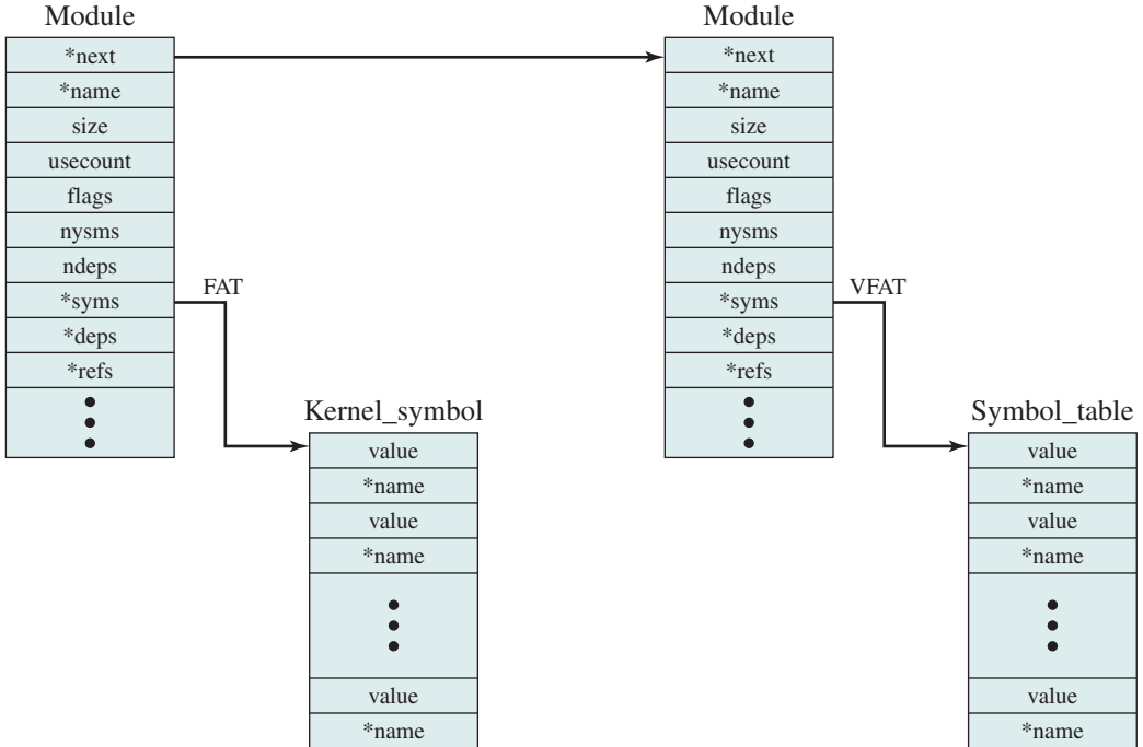
Figure 2.18 Example List of Linux Kernel Modules
