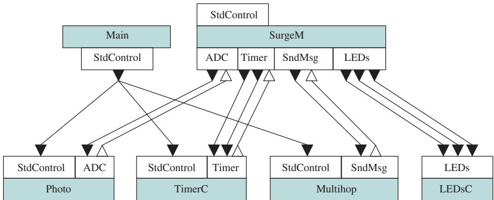
(b) Top-level surge configuration
