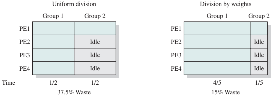
Figure 10.2 Example of Scheduling Groups with Four and One Threads [FEIT90b]
