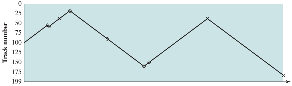
Time (a) FIFO
