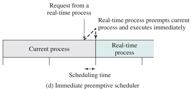
Figure 10.4 Scheduling of Real-Time Process
