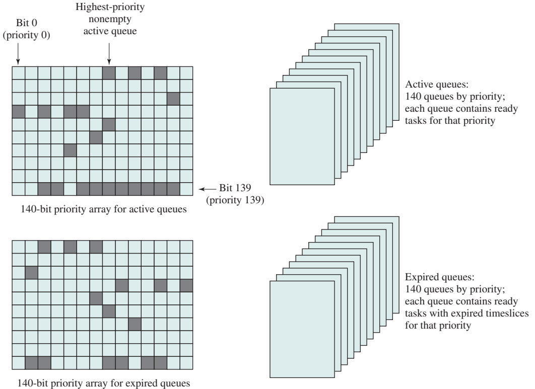
Figure 10.11 Linux Scheduling Data Structures for Each Processor
