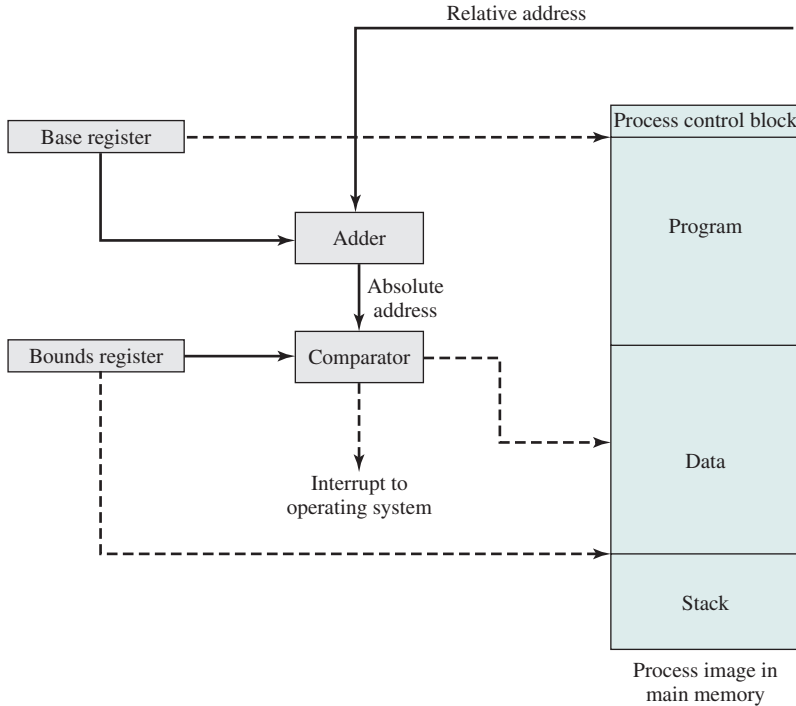
Figure 7.8 Hardware Support for Relocation
