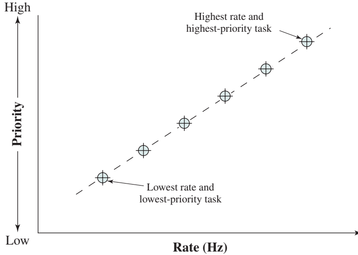
Figure 10.7 A Task Set with RMS [WARR91]
