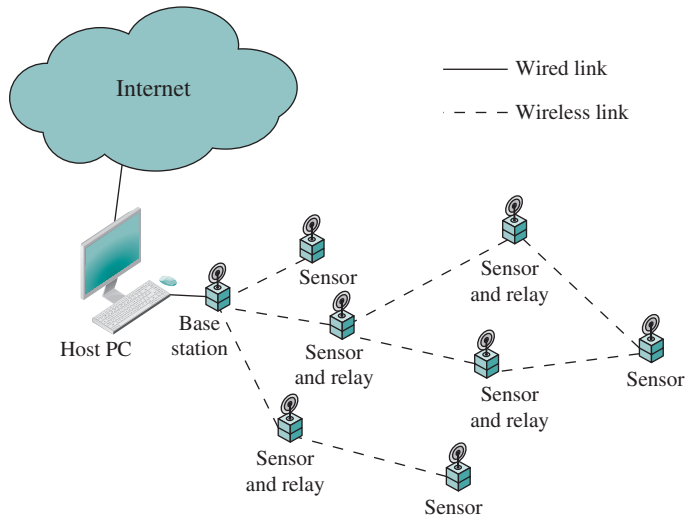
Figure 13.2 Typical Wireless Sensor Network Topology
