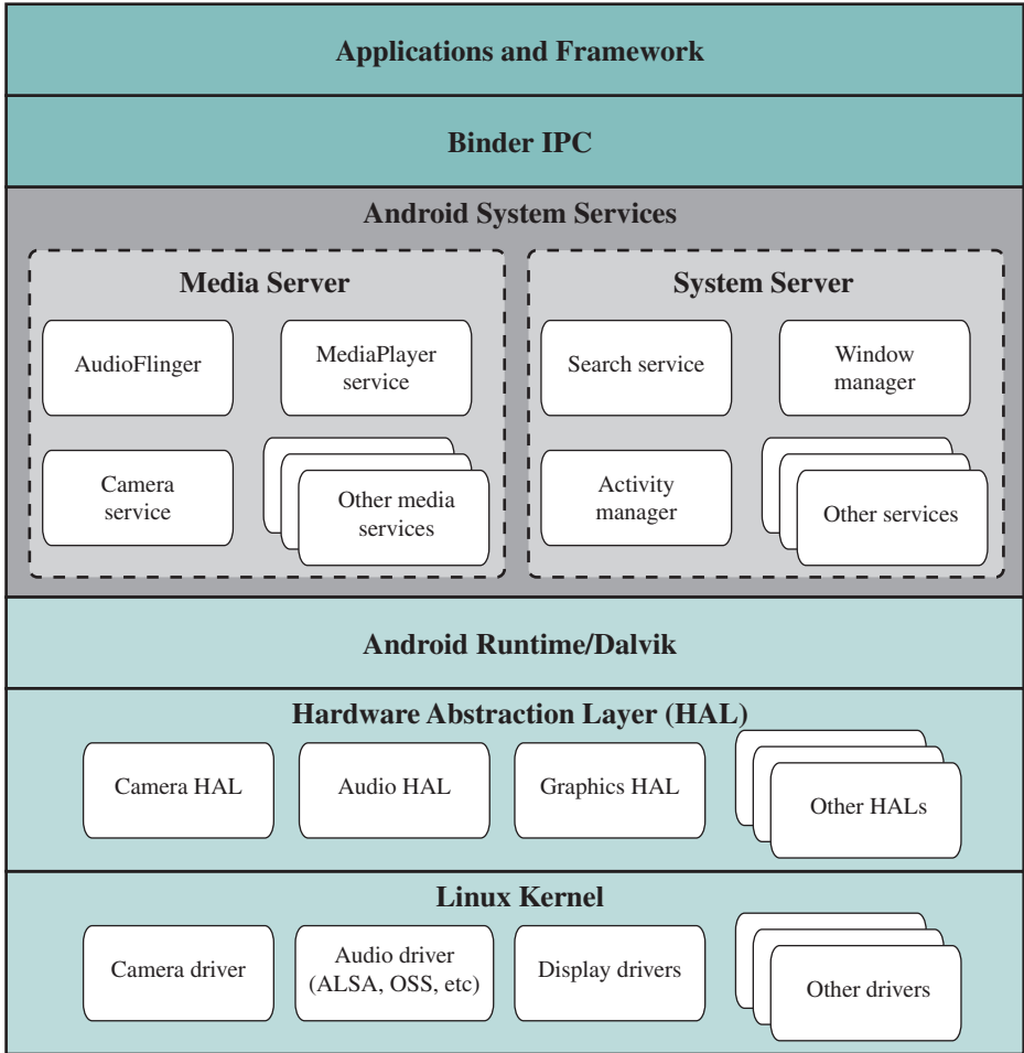
Figure 2.21 Android System Architecture
