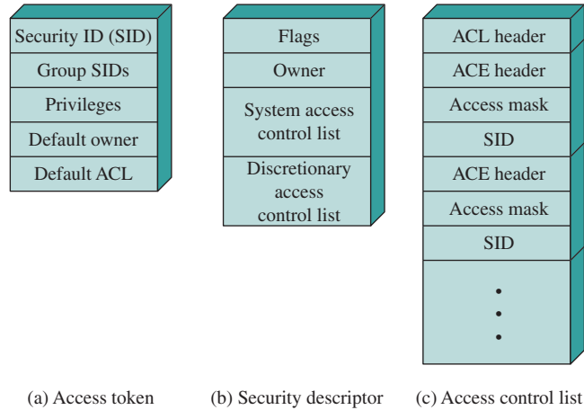
Figure 15.10 Windows Security Structures
