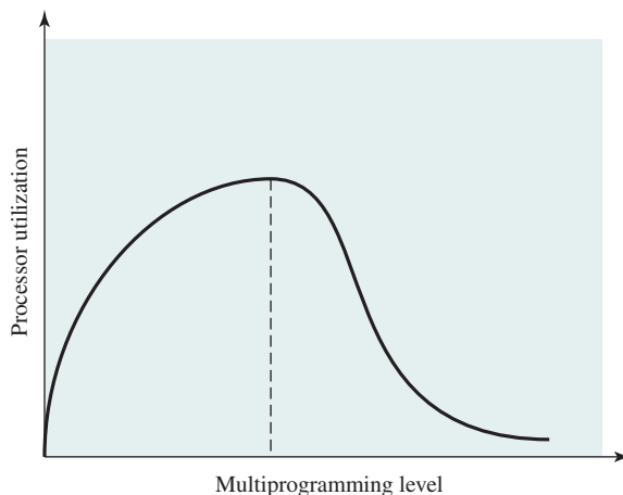
Figure 8.19 Multiprogramming Effects
