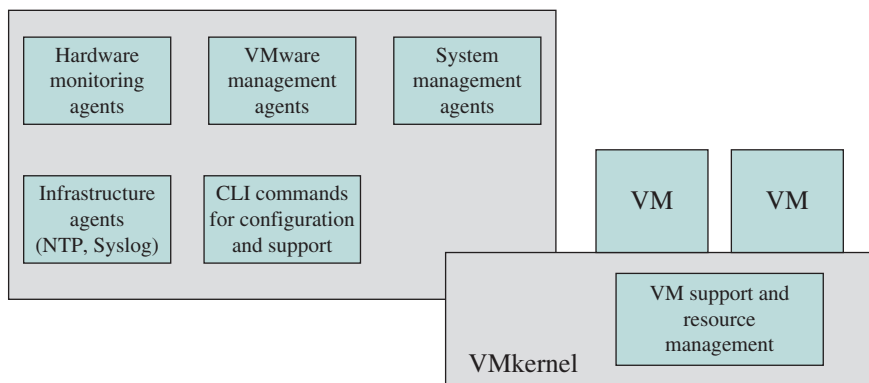
Figure 14.6 ESX
