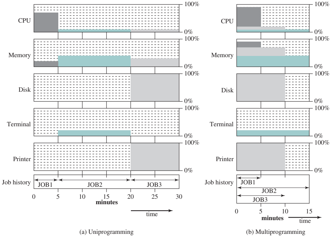
Figure 2.6 Utilization Histograms
