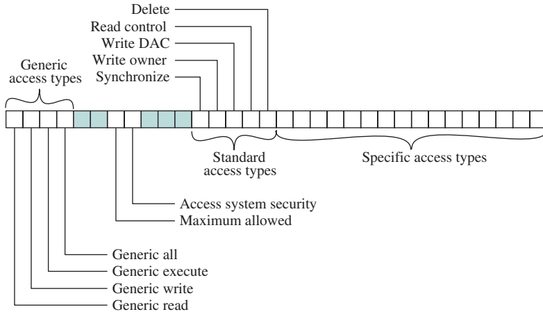
Figure 15.11 Access Mask
