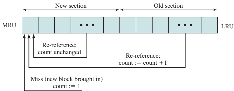
(a) FIFO
