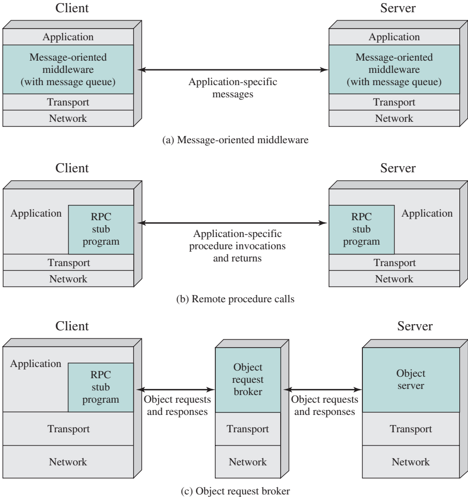
Figure 16.10 Middleware Mechanisms
