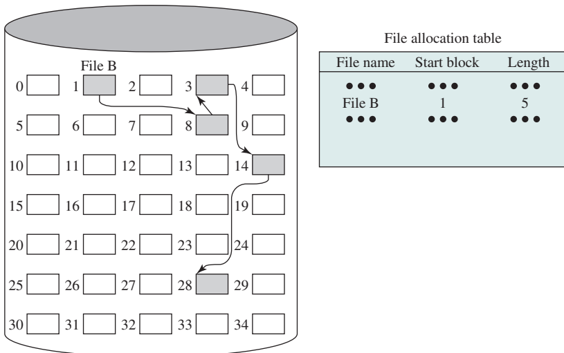
Figure 12.11 Chained Allocation
