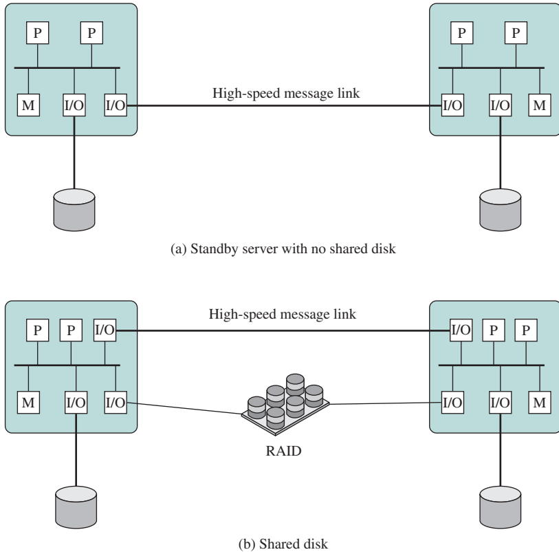
Figure 16.13 Cluster Configurations
