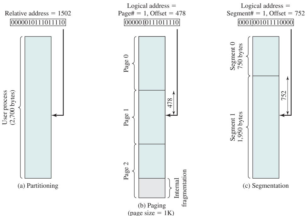
Figure 7.11 Logical Addresses
