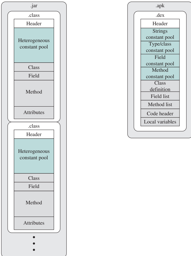
Figure 14.12 Java and Dalvik Formats
