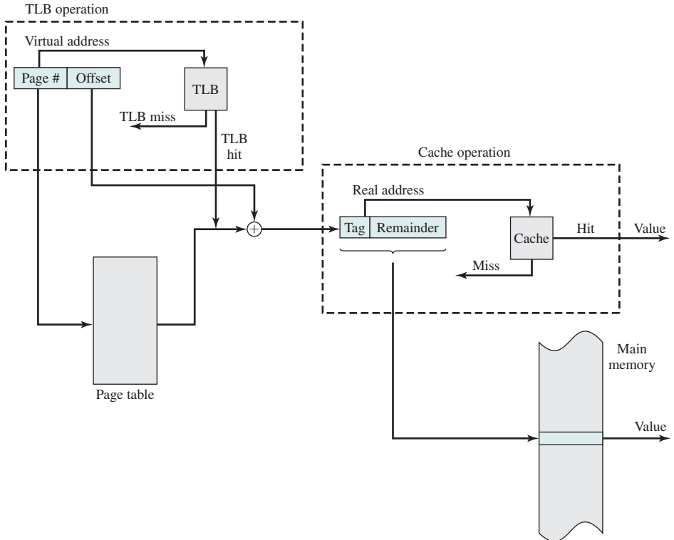
Figure 8.9 Translation Lookaside Buffer and Cache Operation
