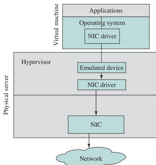
Figure 14.5 I/O in a Virtual Environment
