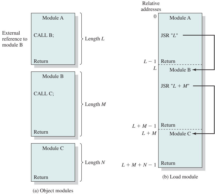
Figure 7.16 The Linking Function
