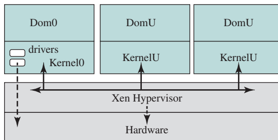
Figure 14.8 Xen
