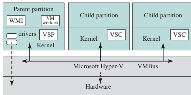
Figure 14.9 Hyper-V
