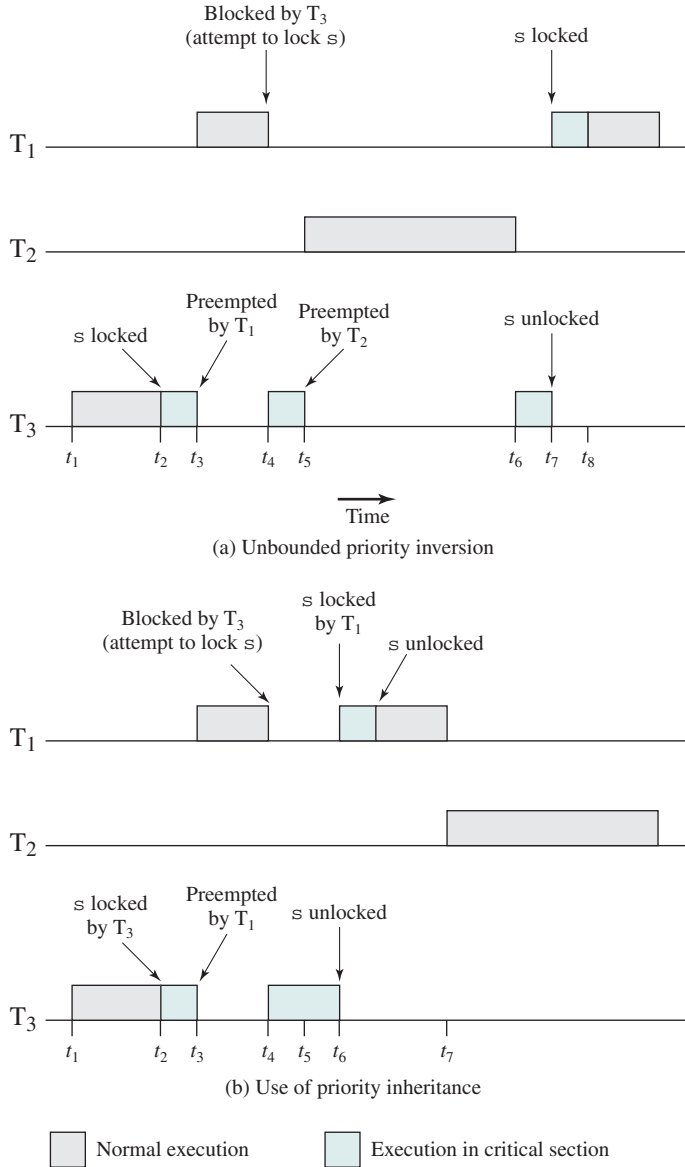
Figure 10.9 Priority Inversion
