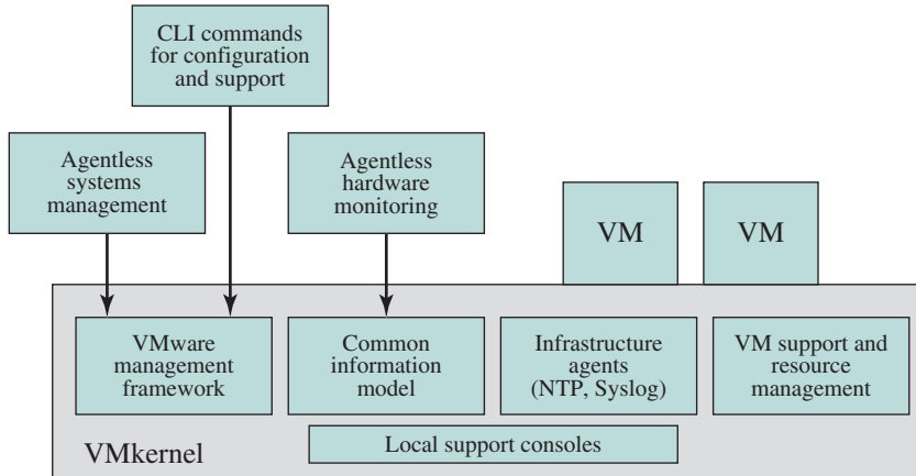
Figure 14.7 ESXi
