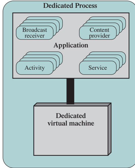
Figure 4.16 Android Application
