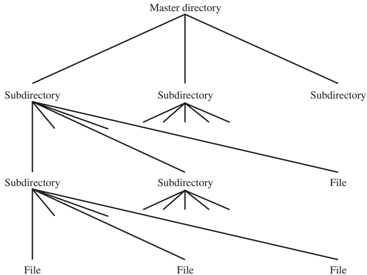
Figure 12.6 Tree-Structured Directory
