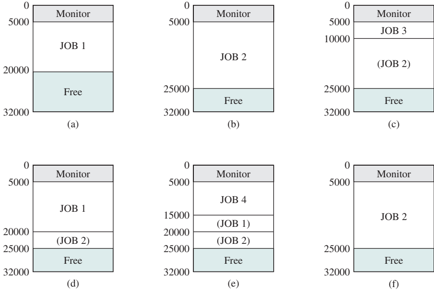
Figure 2.7 CTSS Operation
