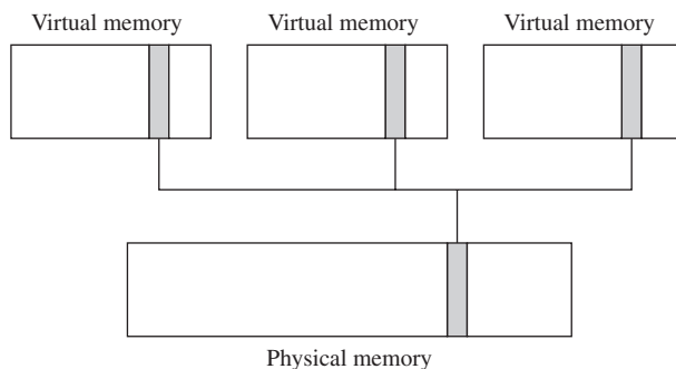
Figure 14.4 Page Sharing
