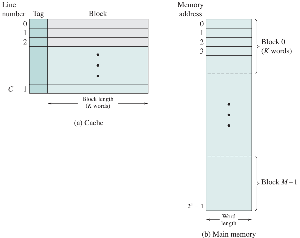
Figure 1.17 Cache/Main-Memory Structure
