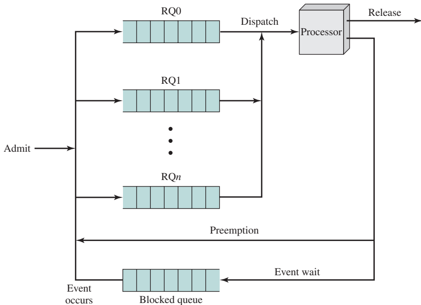
Figure 9.4 Priority Queueing
