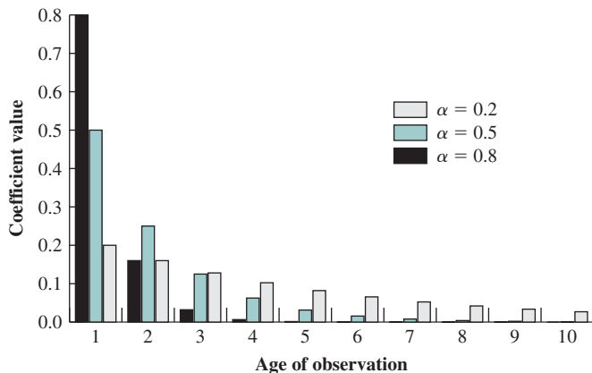
Figure 9.8 Exponential Smoothing Coefficients
