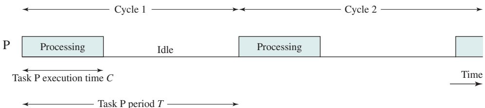
Figure 10.8 Periodic Task Timing Diagram
