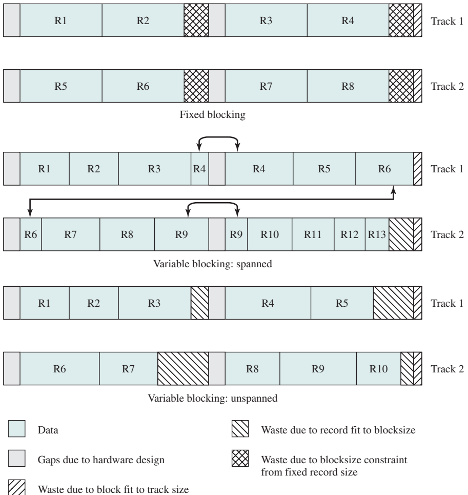
Figure 12.8 Record Blocking Methods [WIED87]
