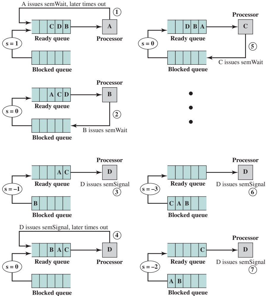
Figure 5.5 Example of Semaphore Mechanism
