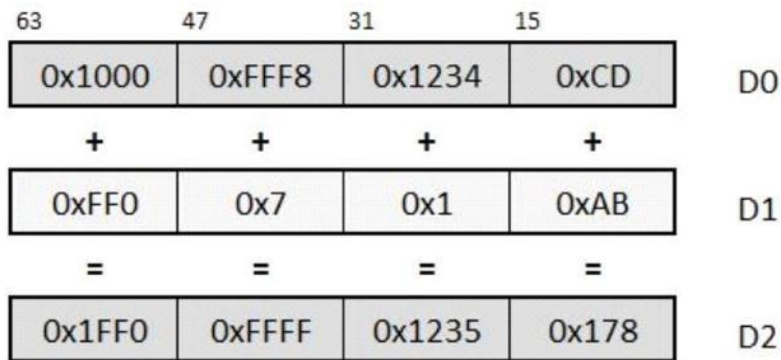
Figure 26e. Adding lane data in Neon.
