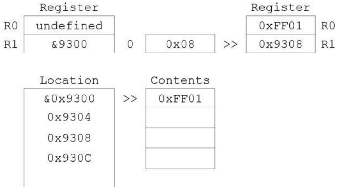
Figure 15e. Post-indexed addressing process.
