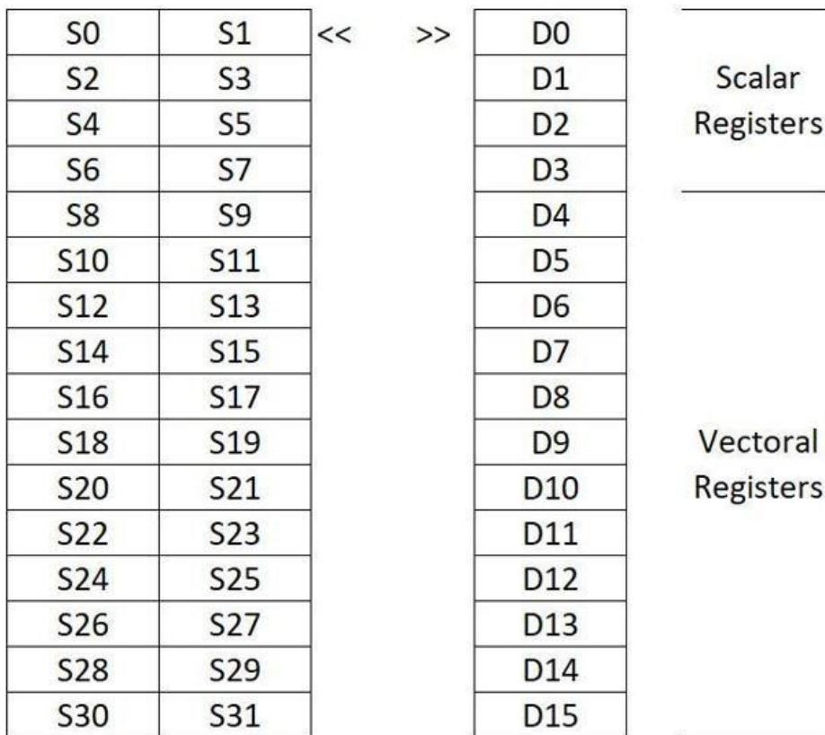
Figure 24b. The VFP Register File. The Sx registers may be used individually or paired to create a double-precision register, Dx.
