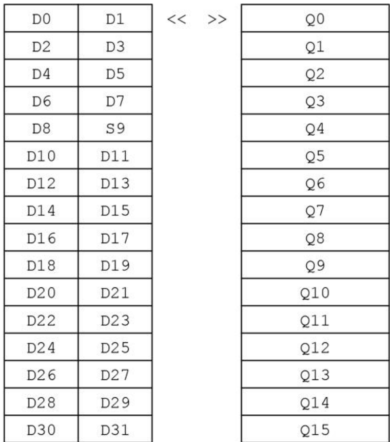
Figure 26b. The Neon register configuration. Compare this to Figure 22b to see how the register structure is built.
