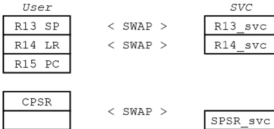
Figure 29g. Swapping registers on at a privileged exception.
