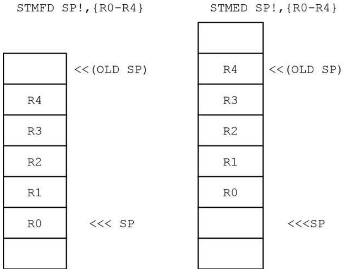
Figure 17e. Full and empty descending stacks.
