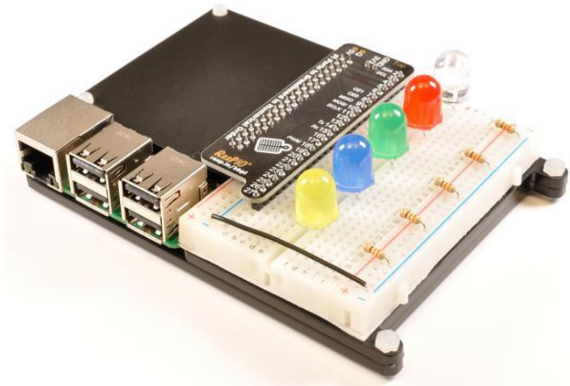
Figure 23a. The Breadboard Pi Bridge from RasP.io.
