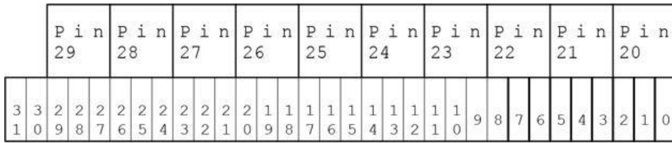
Figure 23c. Bit association with GPSEL2.
