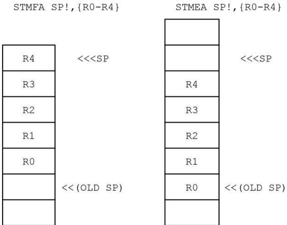
Figure 17d. Full and empty ascending stacks.
