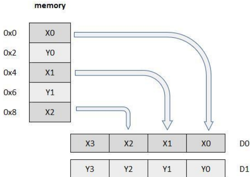
Figure 26f. Selectively loading data into registers with VLD2.16 {D0, D1},[R0].
