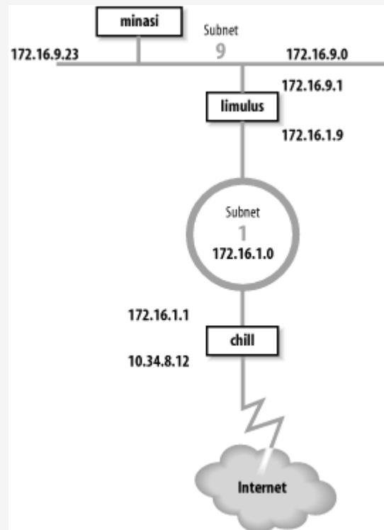
Figure 7-4. Sample routing topology
