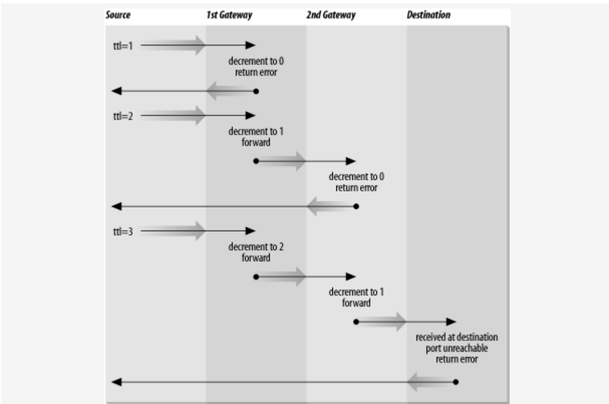
Figure 13-3. Flow of traceroute packets
