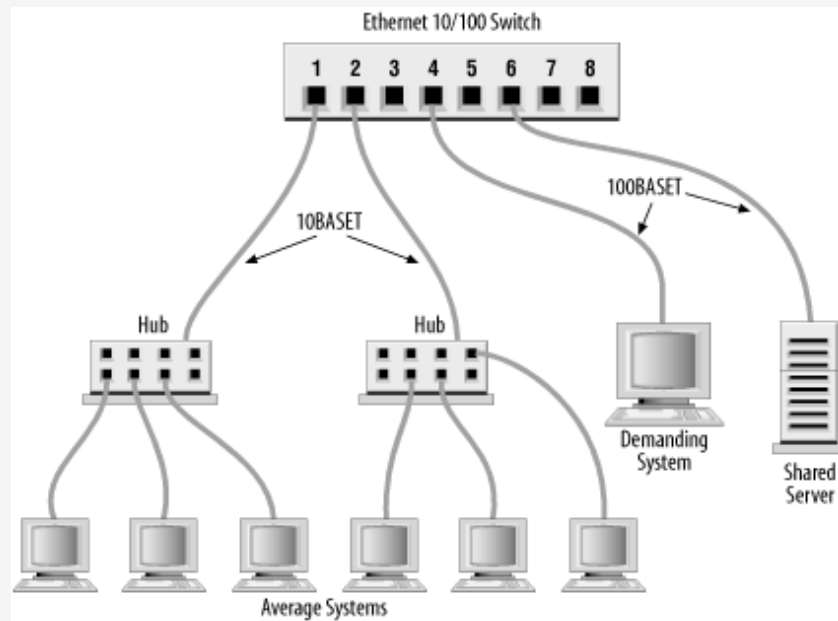
Figure 13-1. Subdividing an Ethernet with switches
