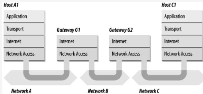
Figure 1-6. Routing through gateways
