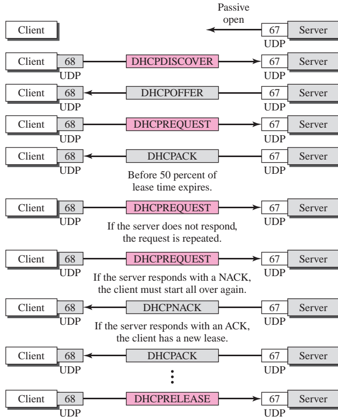
Figure 18.9 Exchanging messages
