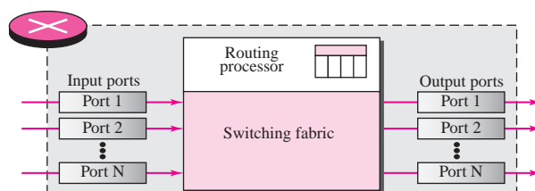
Figure 6.22 Router components
