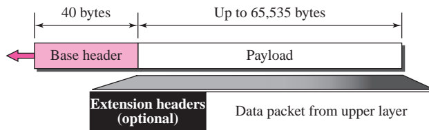
Figure 27.1 IPv6 datagram
