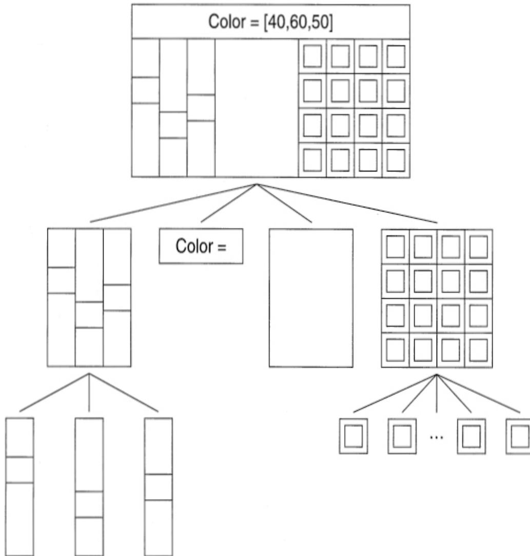
□ Figure 24.1—An example of a Composite
