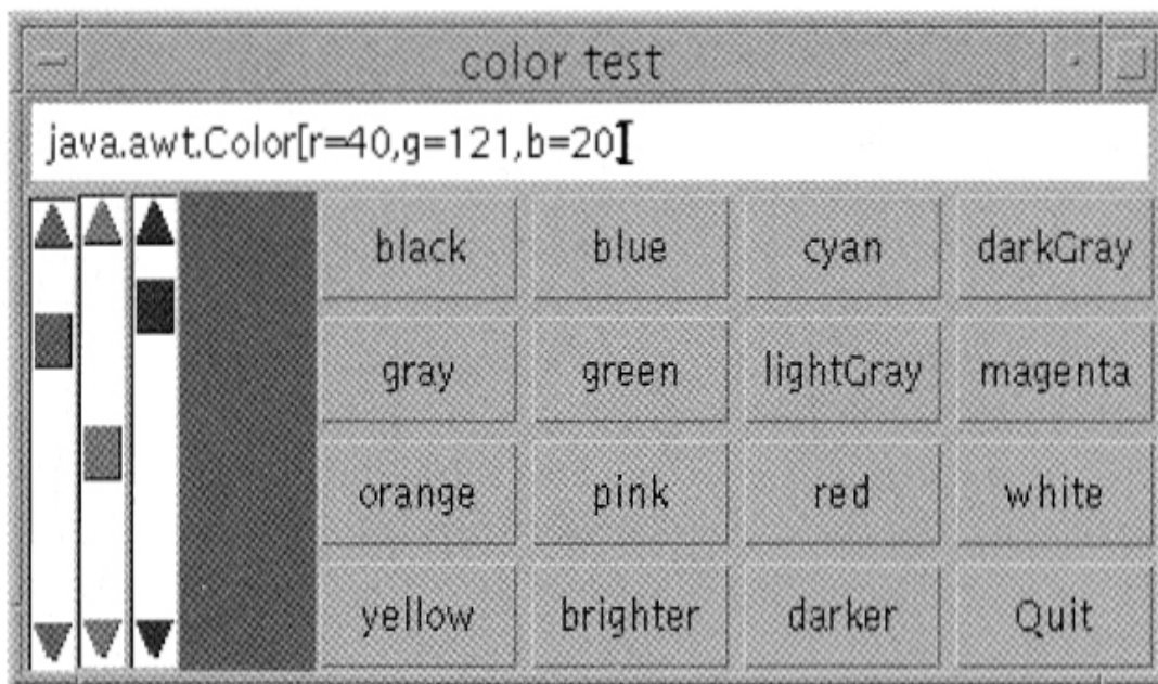
□ Figure 22.4—Snapshot of ColorTest application
