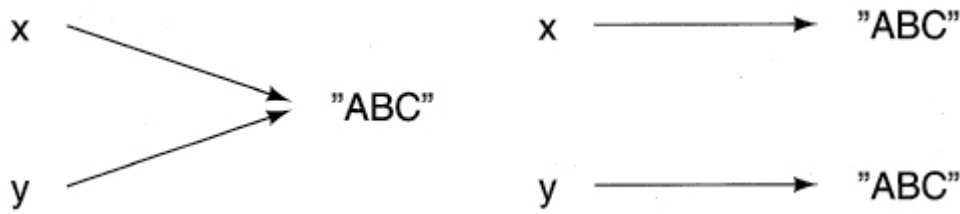
□ Figure 12.3—Identity and equality for character strings
