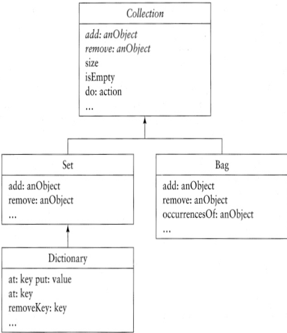
□ Figure 19.1—A portion of the collection inheritance hierarchy in Smalltalk-80
