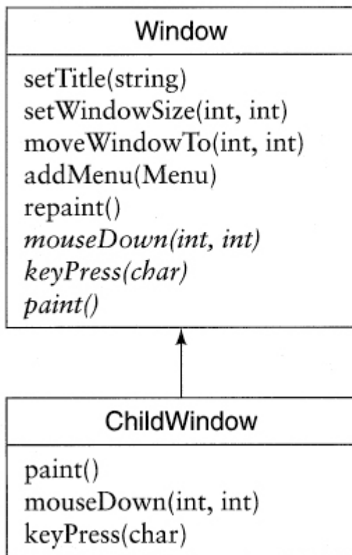
□ Figure 21.1—A GUI class from a typical framework
