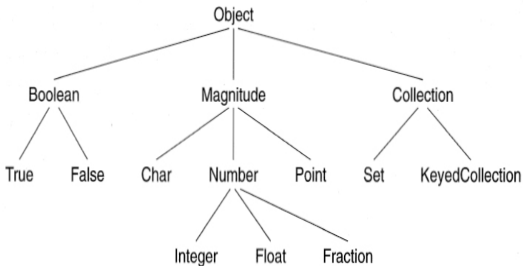
□ Figure 13.1 — A portion of the Smalltalk class hierarchy
