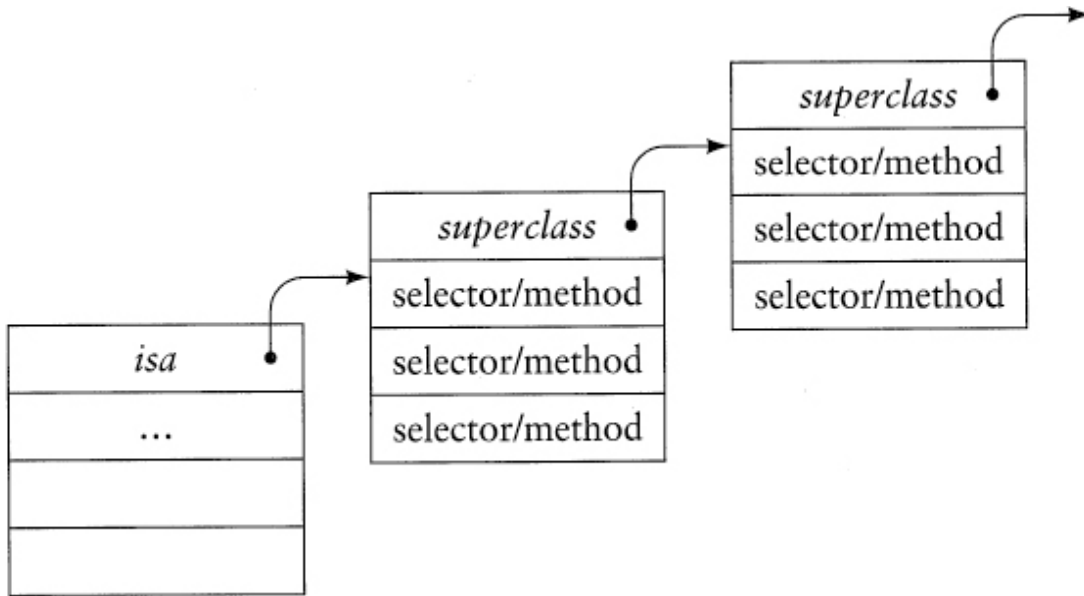
□ Figure 27.1—An object and its dispatch table
