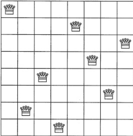
□ Figure 6.1—One solution to the eight-queens puzzle
