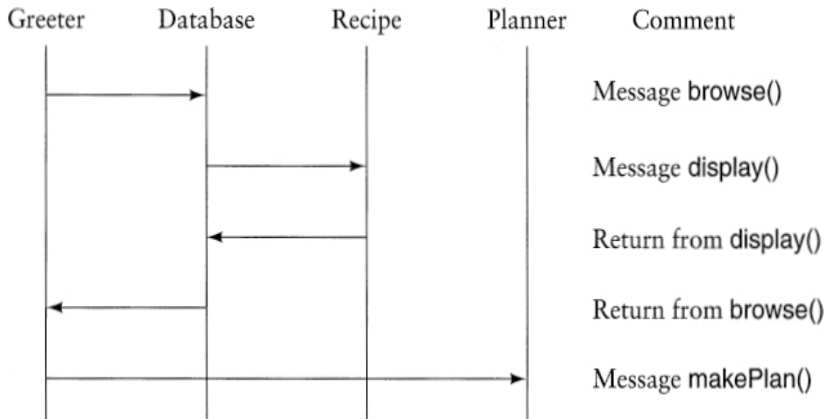
□ Figure 3.5 — An example interaction diagram
