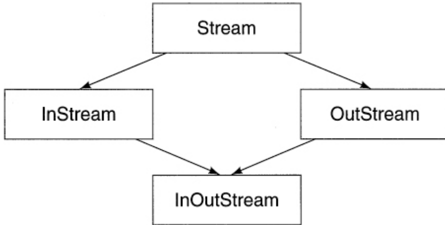
□ Figure 13.3 — An inheritance graph
