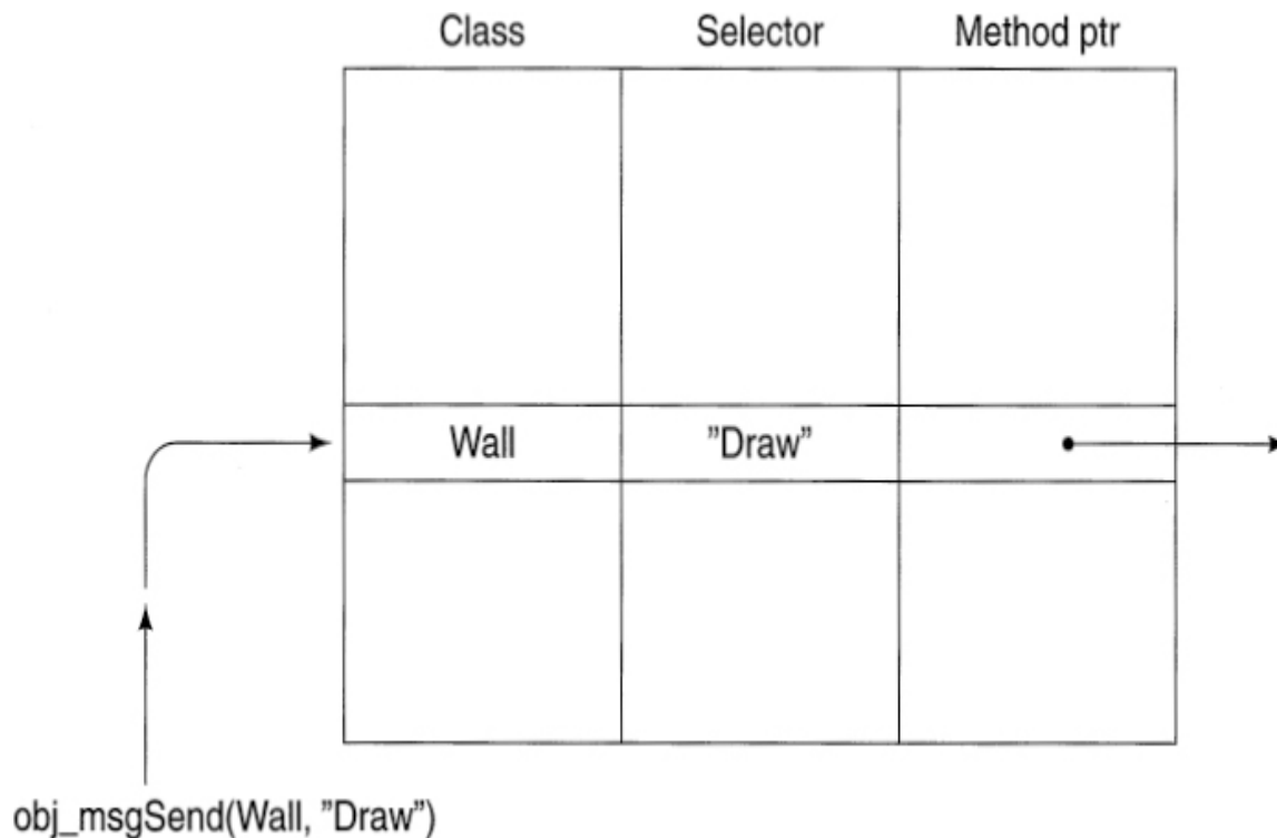
□ Figure 27.2—The messaging function checking the method cache
