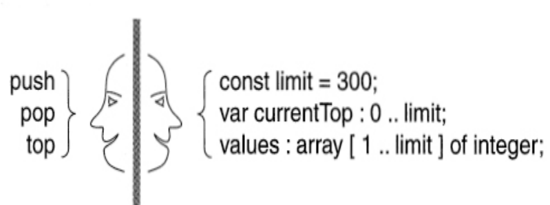
□ Figure 4.1 — The interface and implementation faces of a stack
