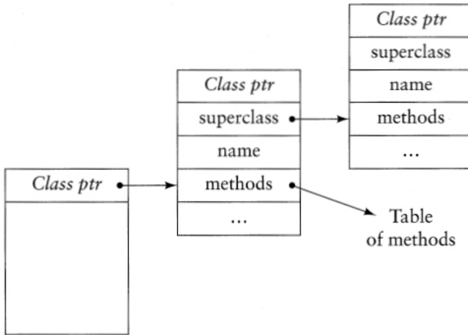
□ Figure 27.4—The internal structure of a class
