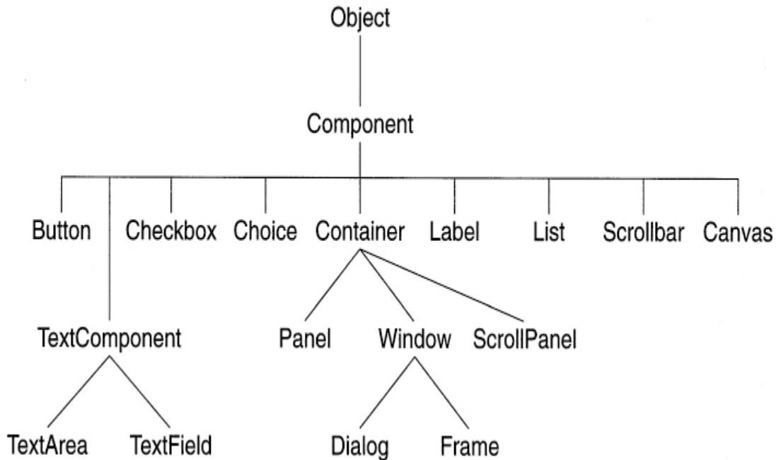
□ Figure 22.1—The AWT class hierarchy
