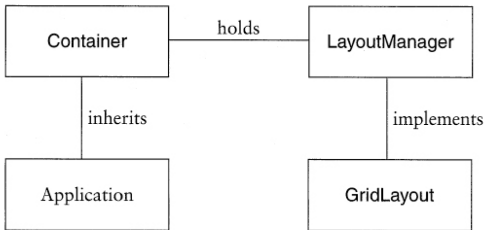
□ Figure 22.3—Relationships between layout manager components
