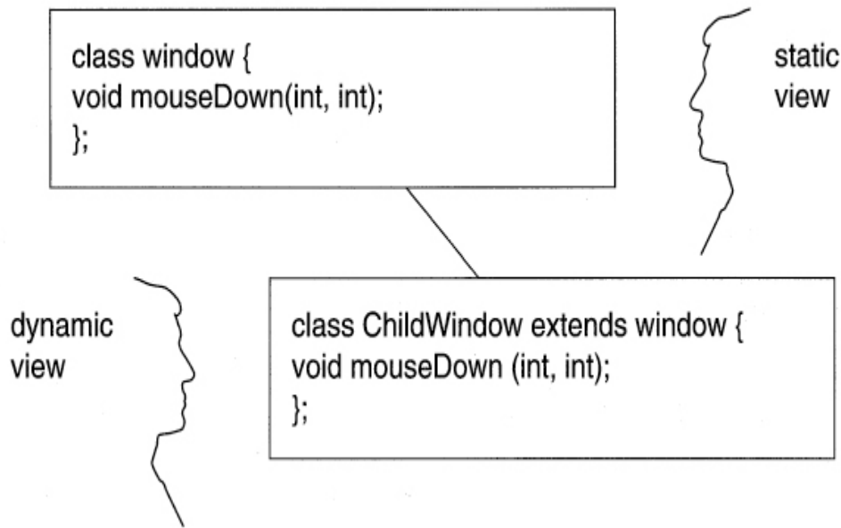
□ Figure 21.2—Two views of the same class.
