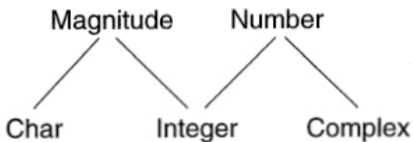
□ Figure 13.2 — A multiple inheritance hierarchy for complex numbers
