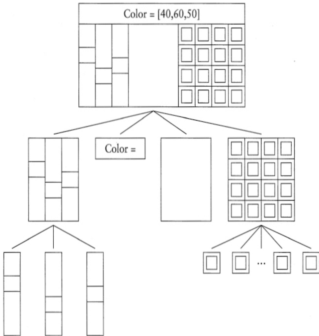
□ Figure 2.3 — Composition in the creation of user interfaces
