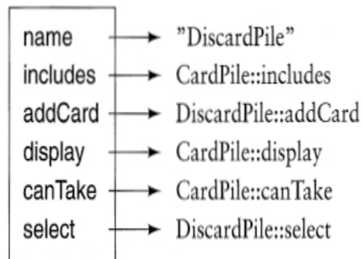
DiscardPile VMT
