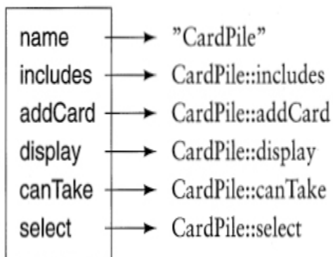
CardPile VMT
