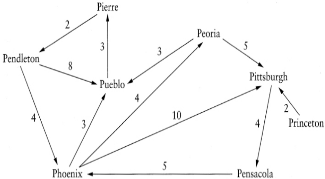
□ Figure 20.1—A Weighted Graph
