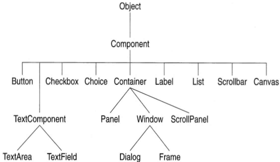
□ Figure 2.4 — The AWT class hierarchy
