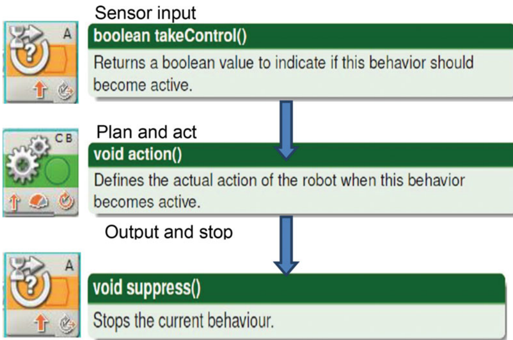
Figure 12-2. Behavior programming
