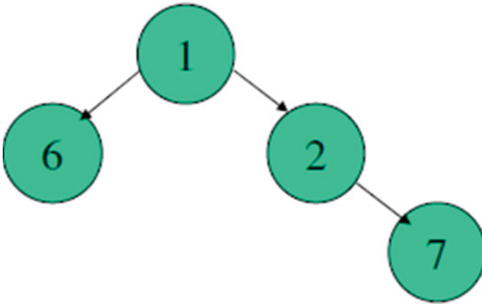
Figure 9-3. Tree structure of nodes after visiting Node 2
